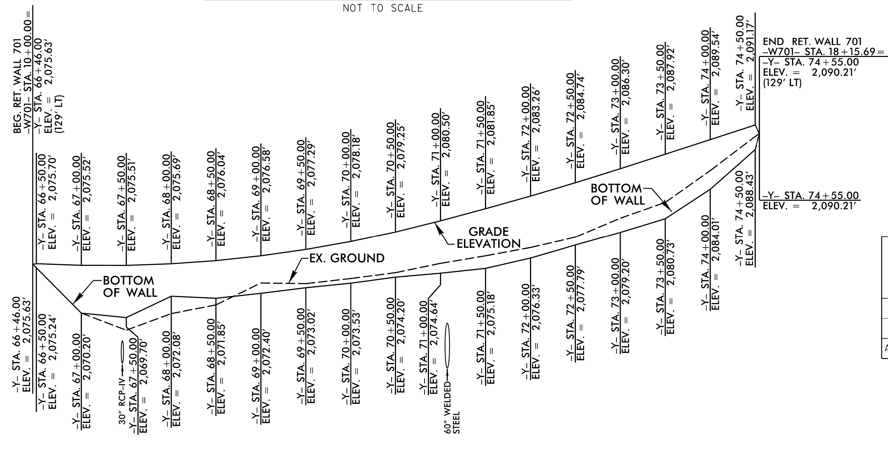
RETAINING WALL NO. W701 ENVELOPE DIMENSIONS OF WALL TAKEN ALONG FRONT FACE OF MSE WALL NOT TO SCALE
