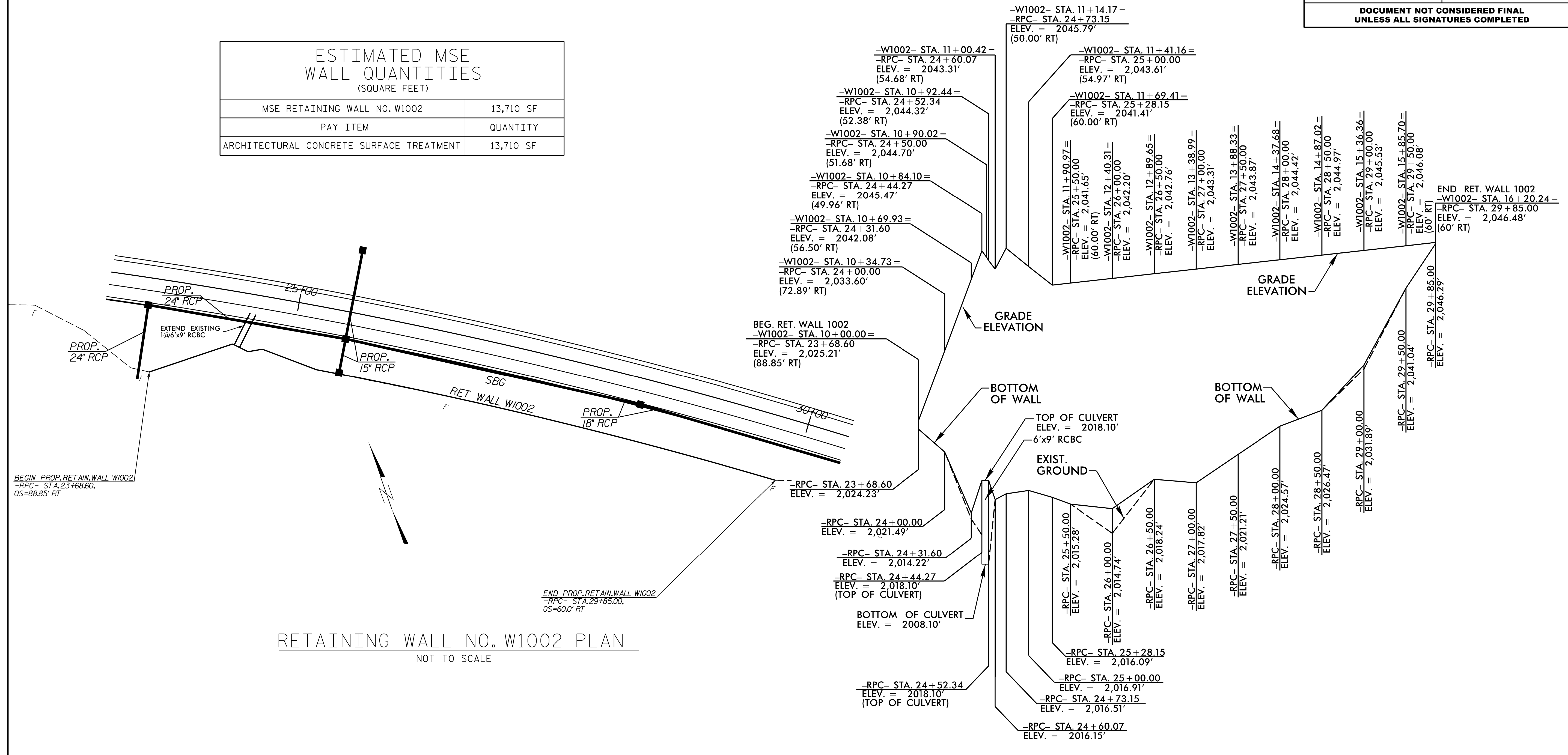
RETAINING WALL NO. W1002 ENVELOPE DIMENSIONS OF WALL TAKEN ALONG FRONT FACE OF MSE WALL NOT TO SCALE
