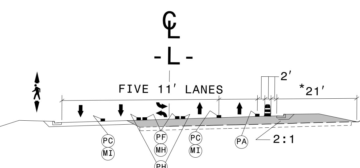
TYPICAL SECTION A-A STA. 17+00+/-
