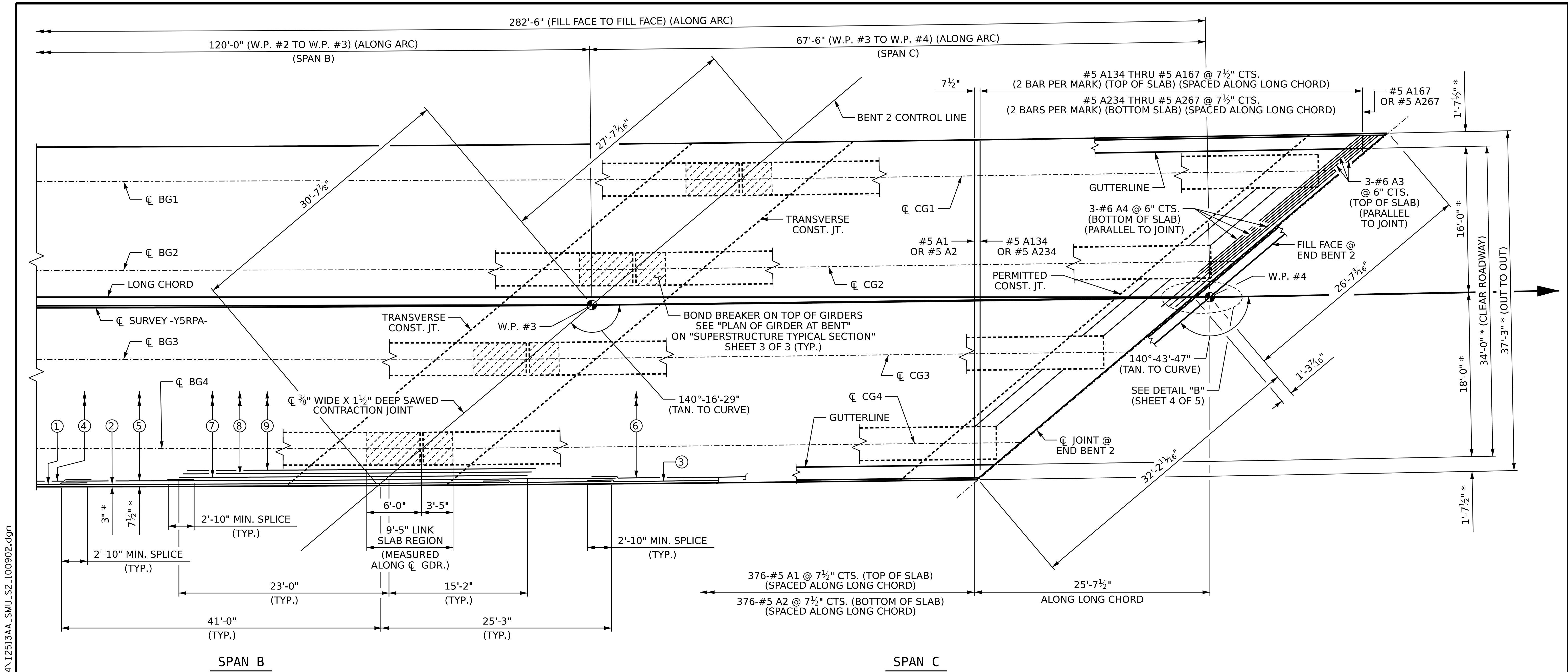
PLAN OF SPANS (TOP & BOTTOM "A" BARS SHOWN) (ONLY TOP "B" BARS SHOWN FOR CLARITY)
