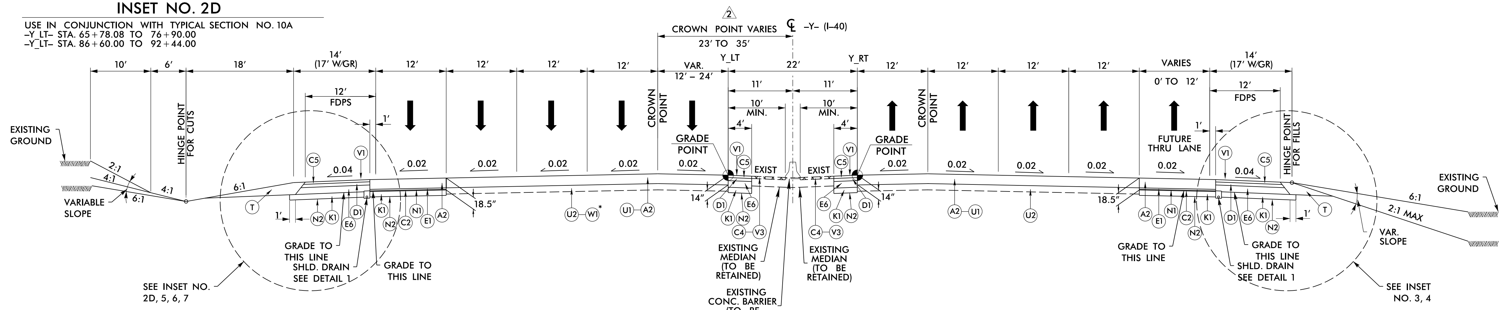
TYPICAL SECTION NO. 10A -Y_LT- STA. 65+78.08 TO 92+44.00 -Y_RT- STA. 63+61.68 (NW5A) TO 92+44.00
