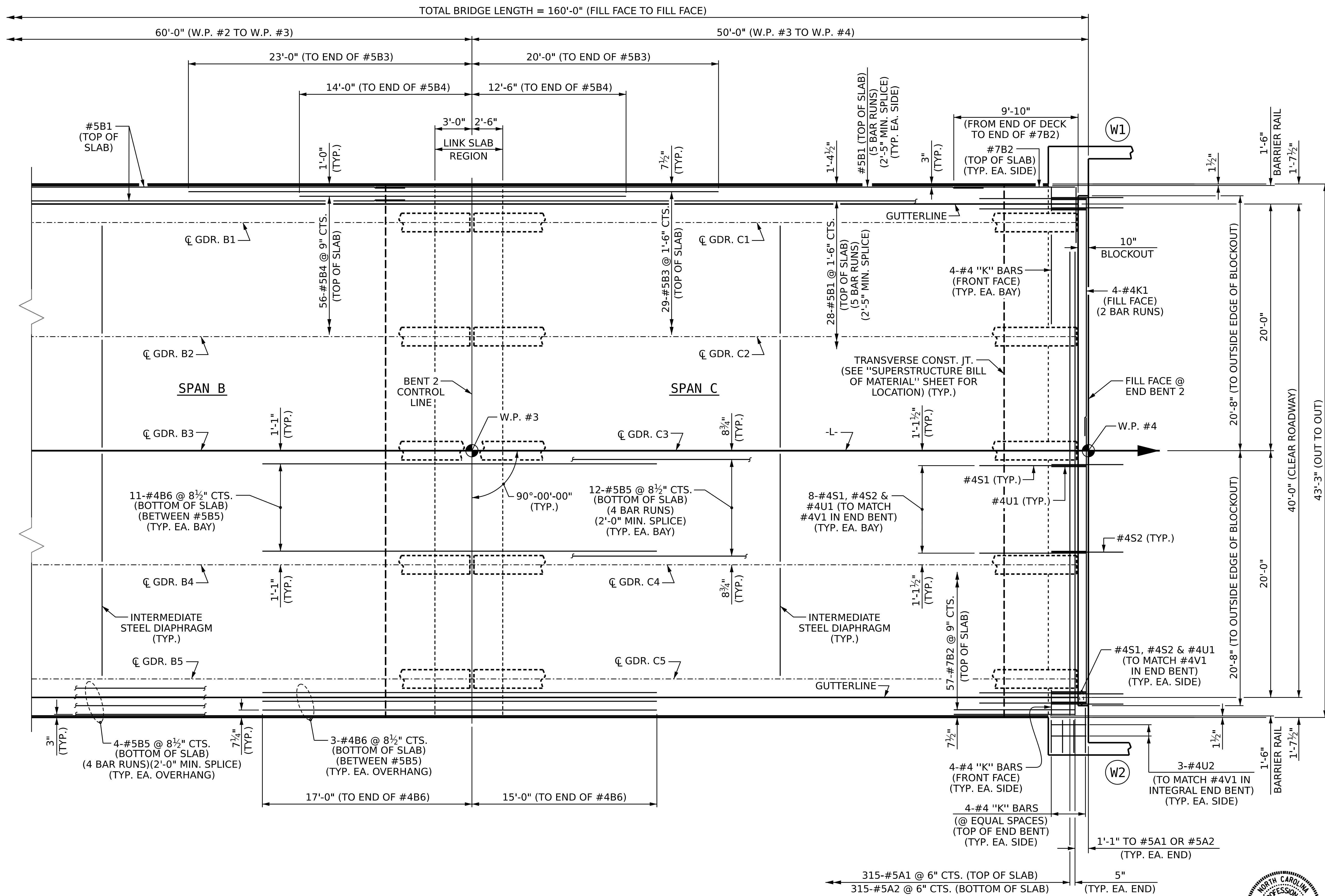
PARTIAL PLAN OF SPAN B
