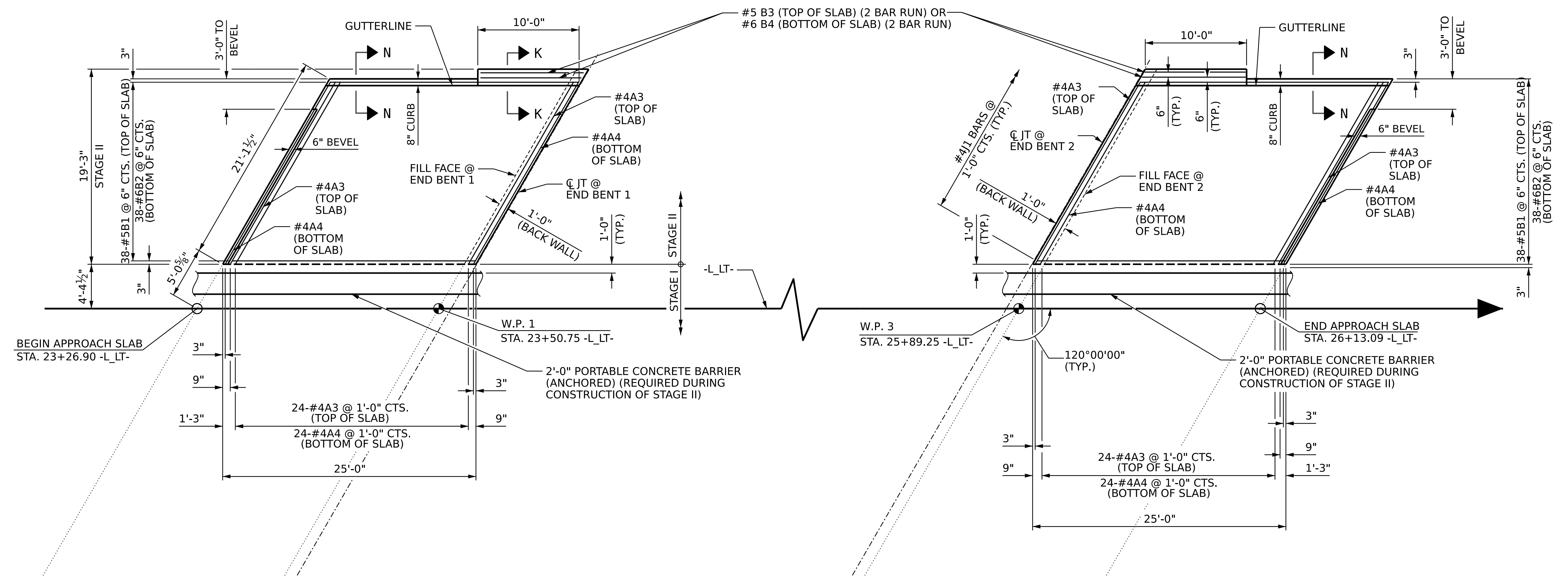
PLAN @ END BENT 1
