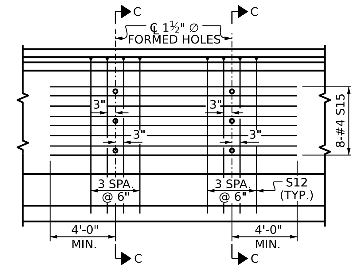
PARTIAL ELEVATION SHOWING INTERMEDIATE STEEL DIAPHRAGM REINFORCING STEEL FOR GIRDER Nos. 2,5,6
