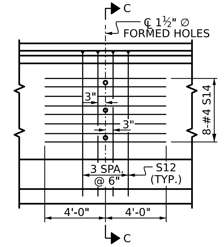
PARTIAL ELEVATION SHOWING INTERMEDIATE STEEL DIAPHRAGM REINFORCING STEEL FOR GIRDER Nos. 1,3,4,7
