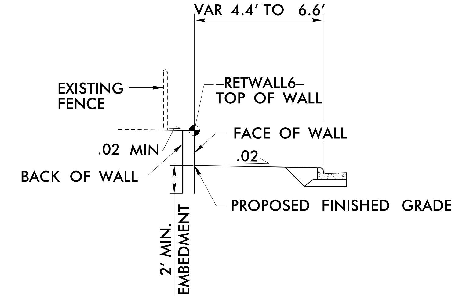
RETAINING WALL DETAIL (-RETWALL6-)
