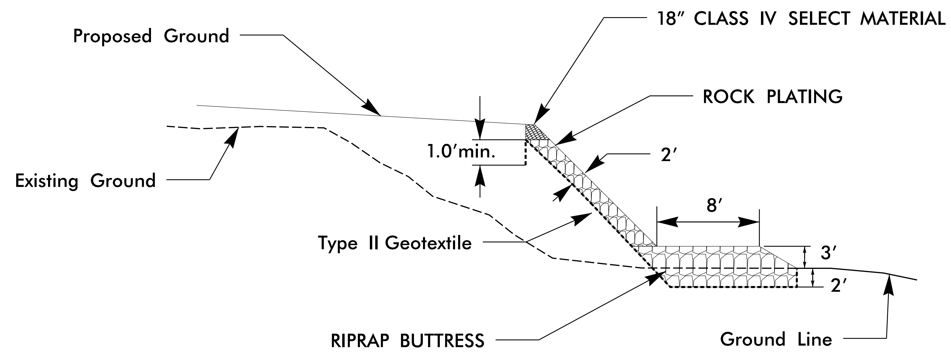
ROCK PLATING AND RIP RAP BUTTRESS TYPICAL SECTION (Not to Scale)
