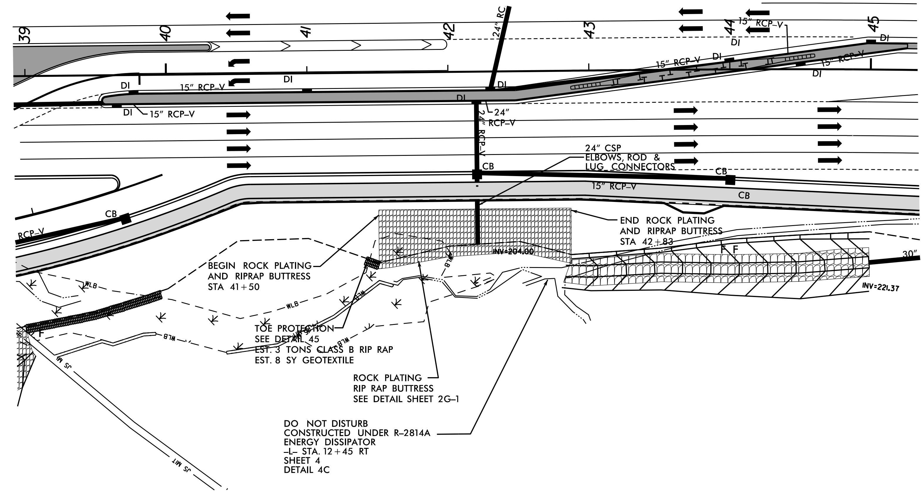
PLAN VIEW (Not to Scale)
