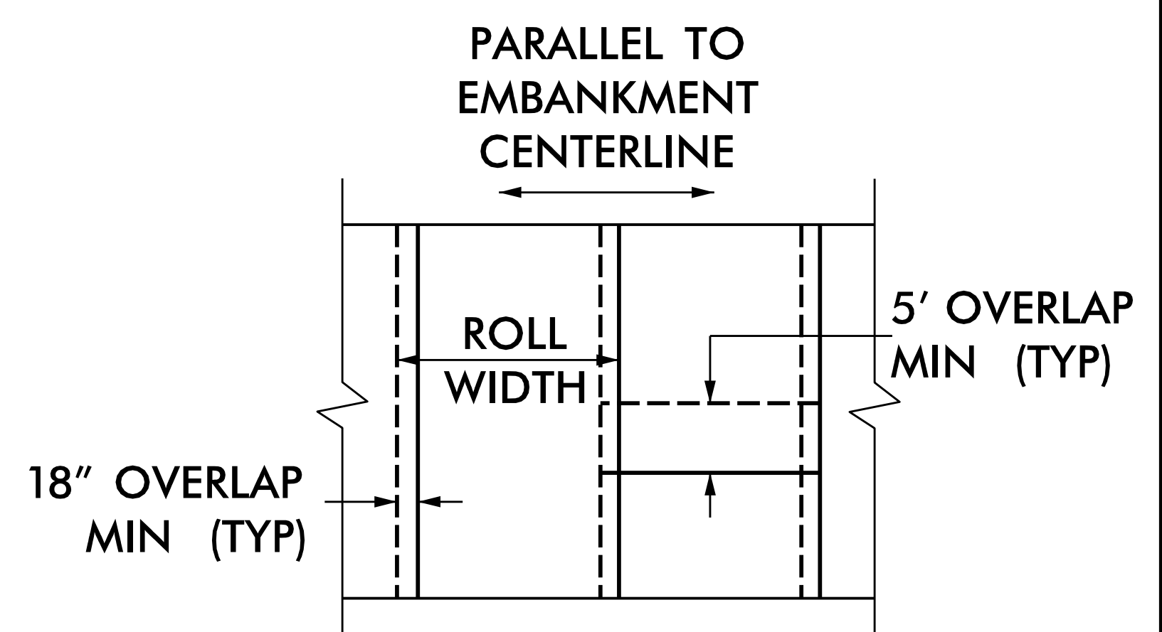
GEOTEXTILE OVERLAP DETAIL (PLAN VIEW, N.T.S.)
