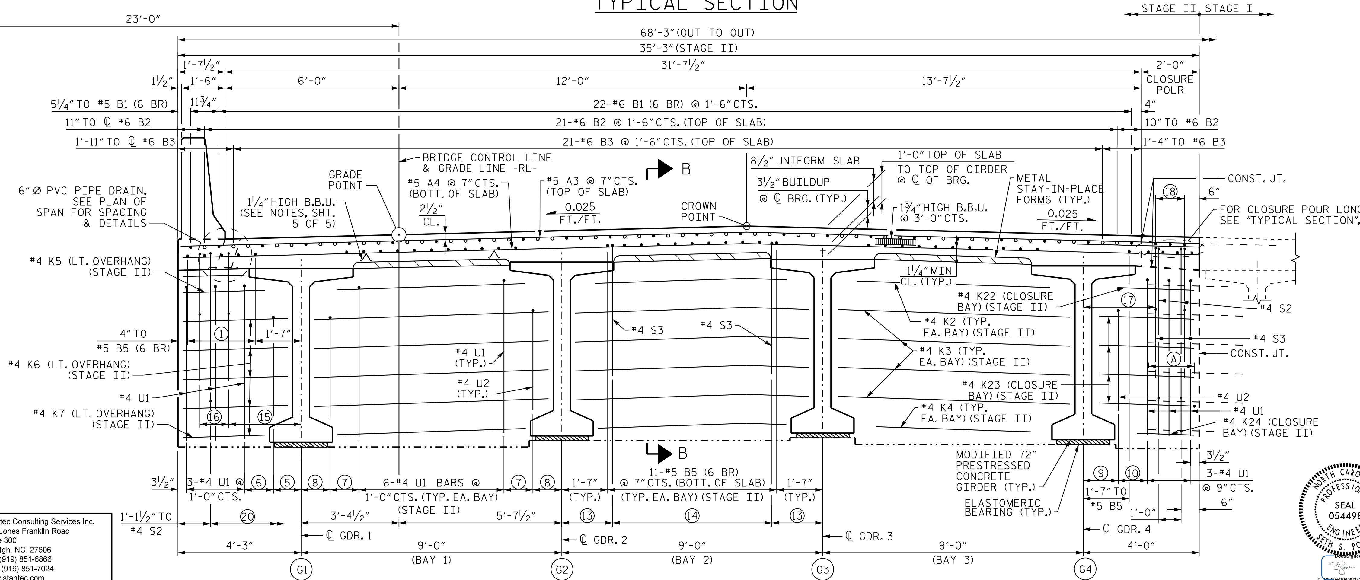
INTEGRAL DIAPHRAGM REINFORCING AT FRONT FACE (STAGE II) TYPICAL SECTION
