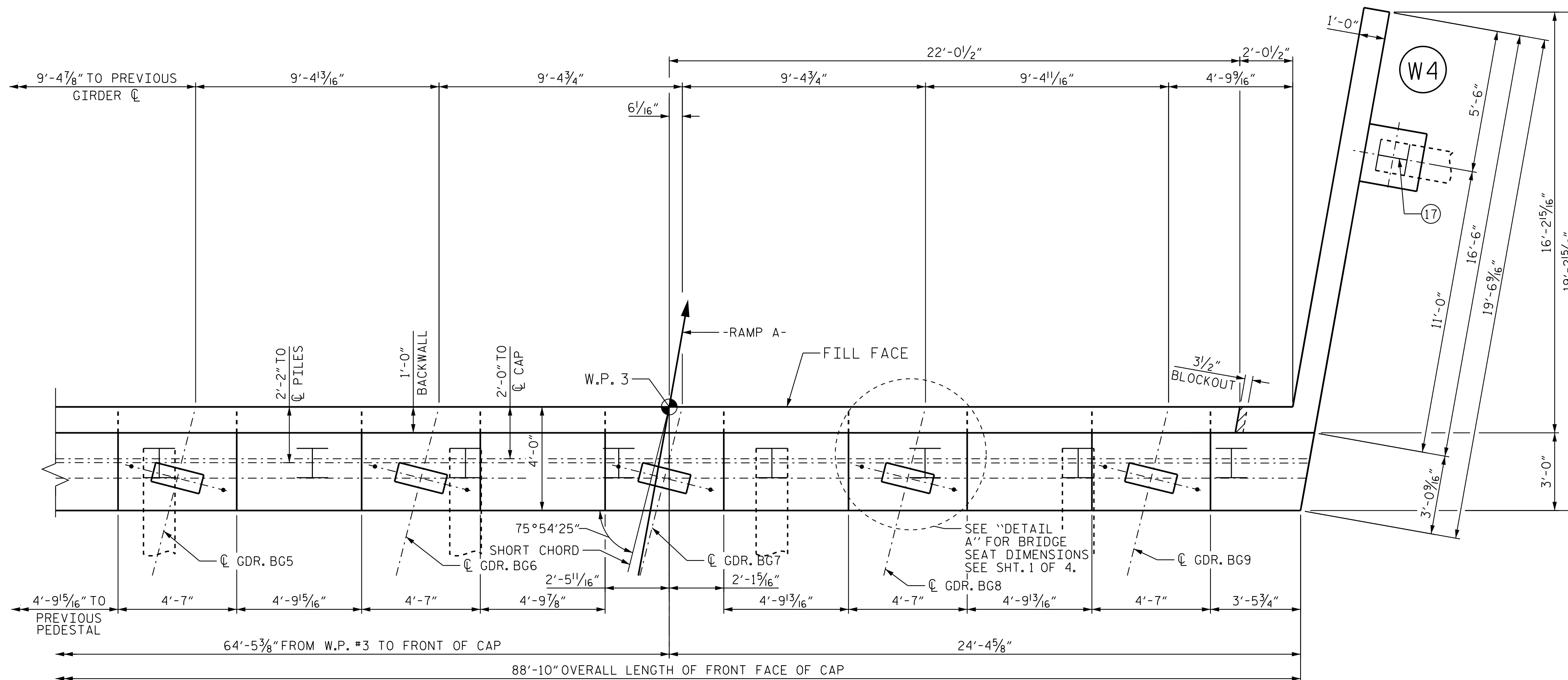
PLAN
