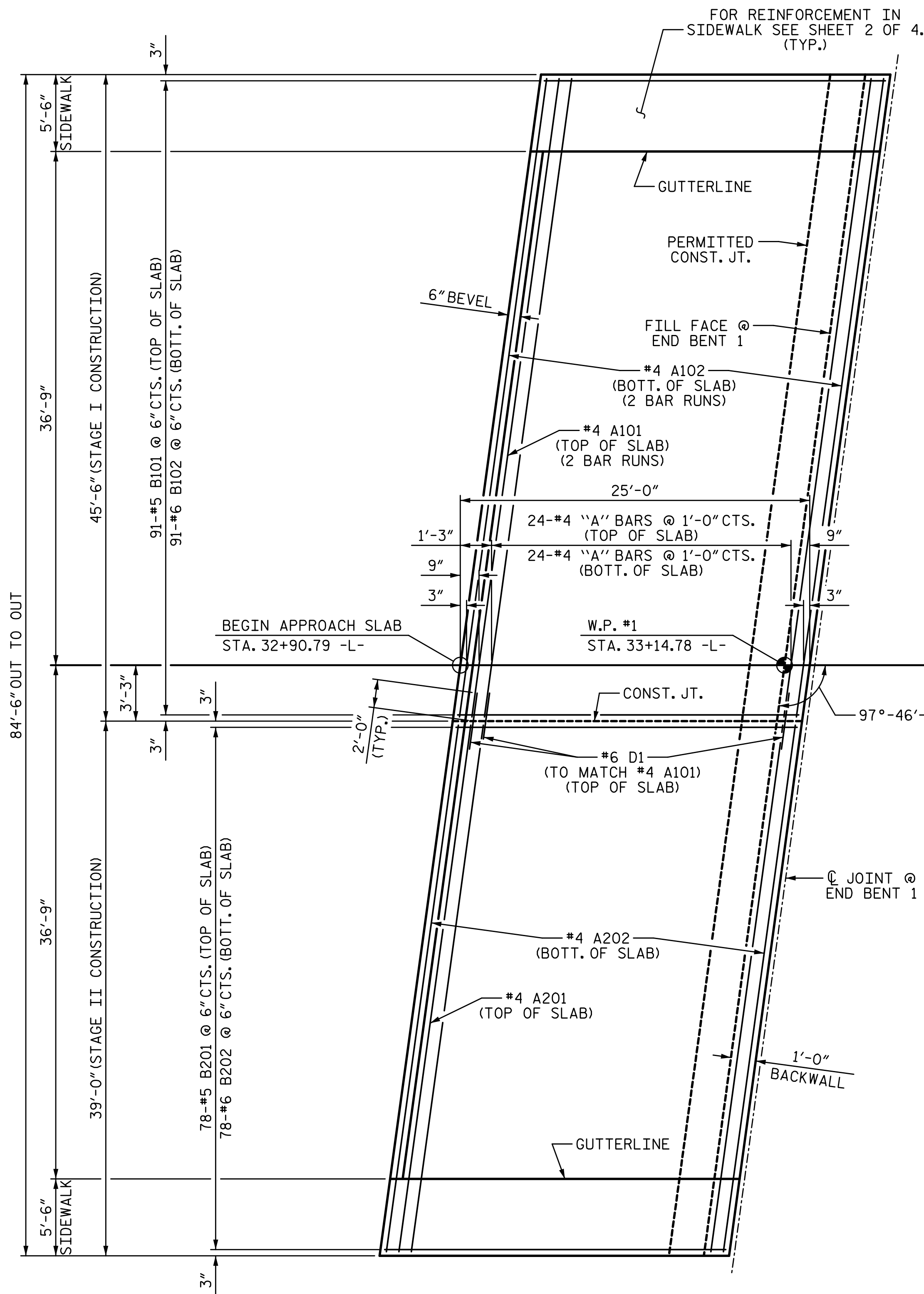
PLAN @ END BENT 1
