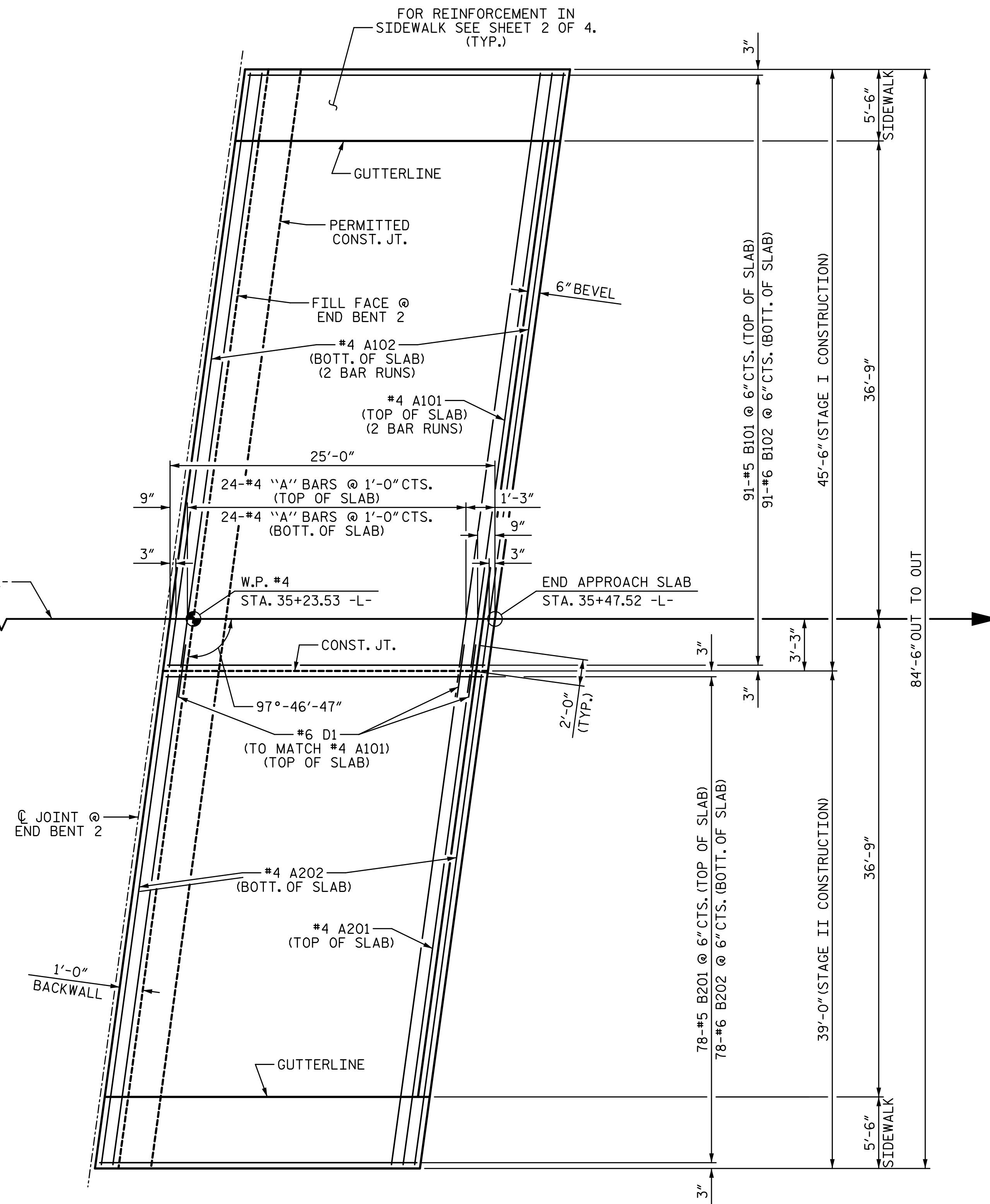
PLAN @ END BENT 2
