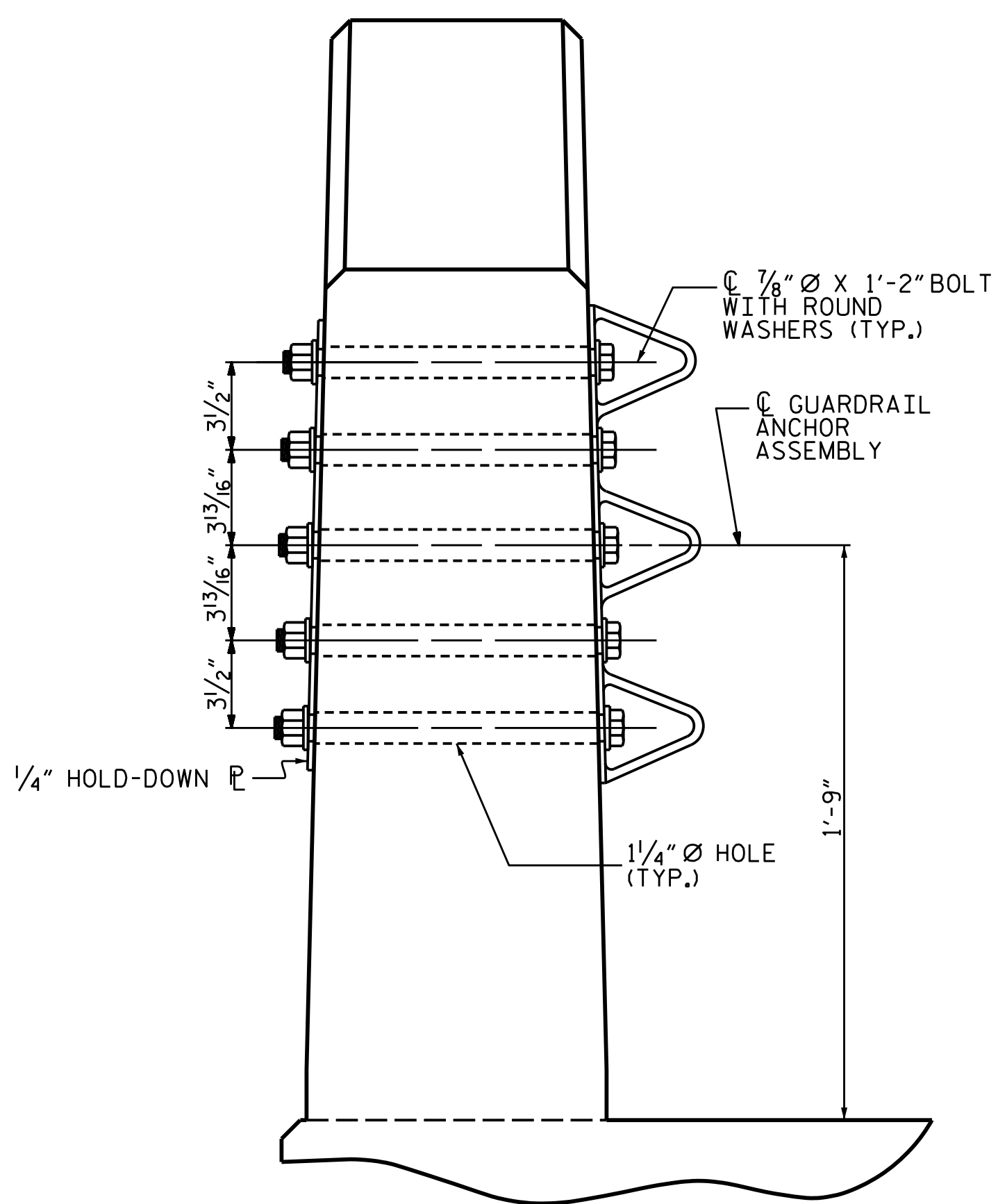
SECTION E-E
