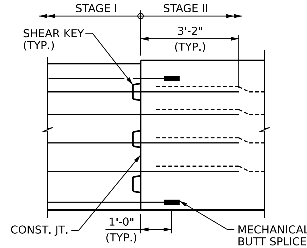
DETAIL "B"
