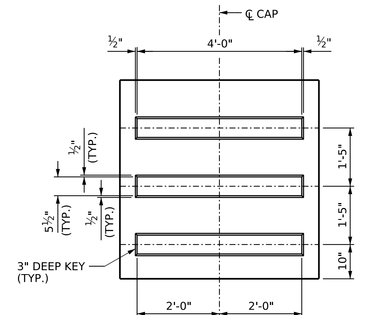
SECTION X-X
