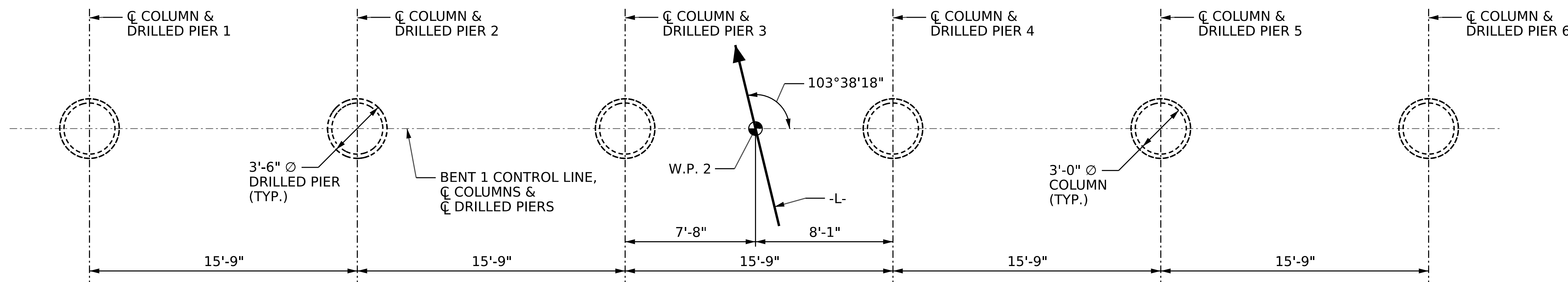
PLAN OF DRILLED PIERS AND COLUMNS
