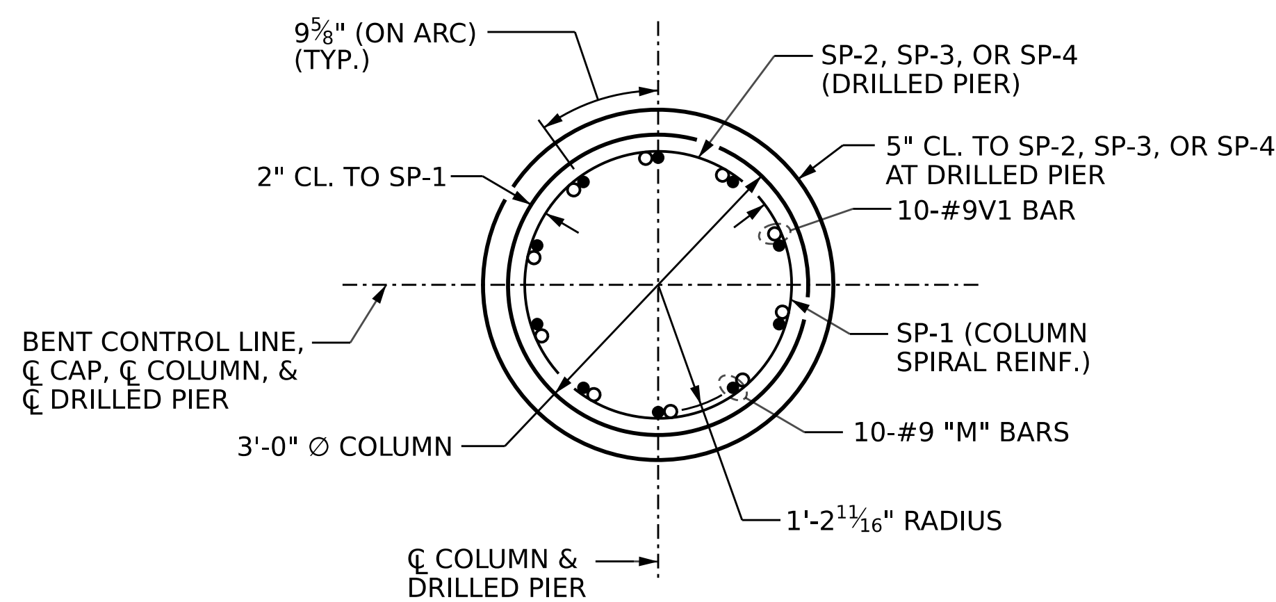
SECTION THRU COLUMN & DRILLED PIER
