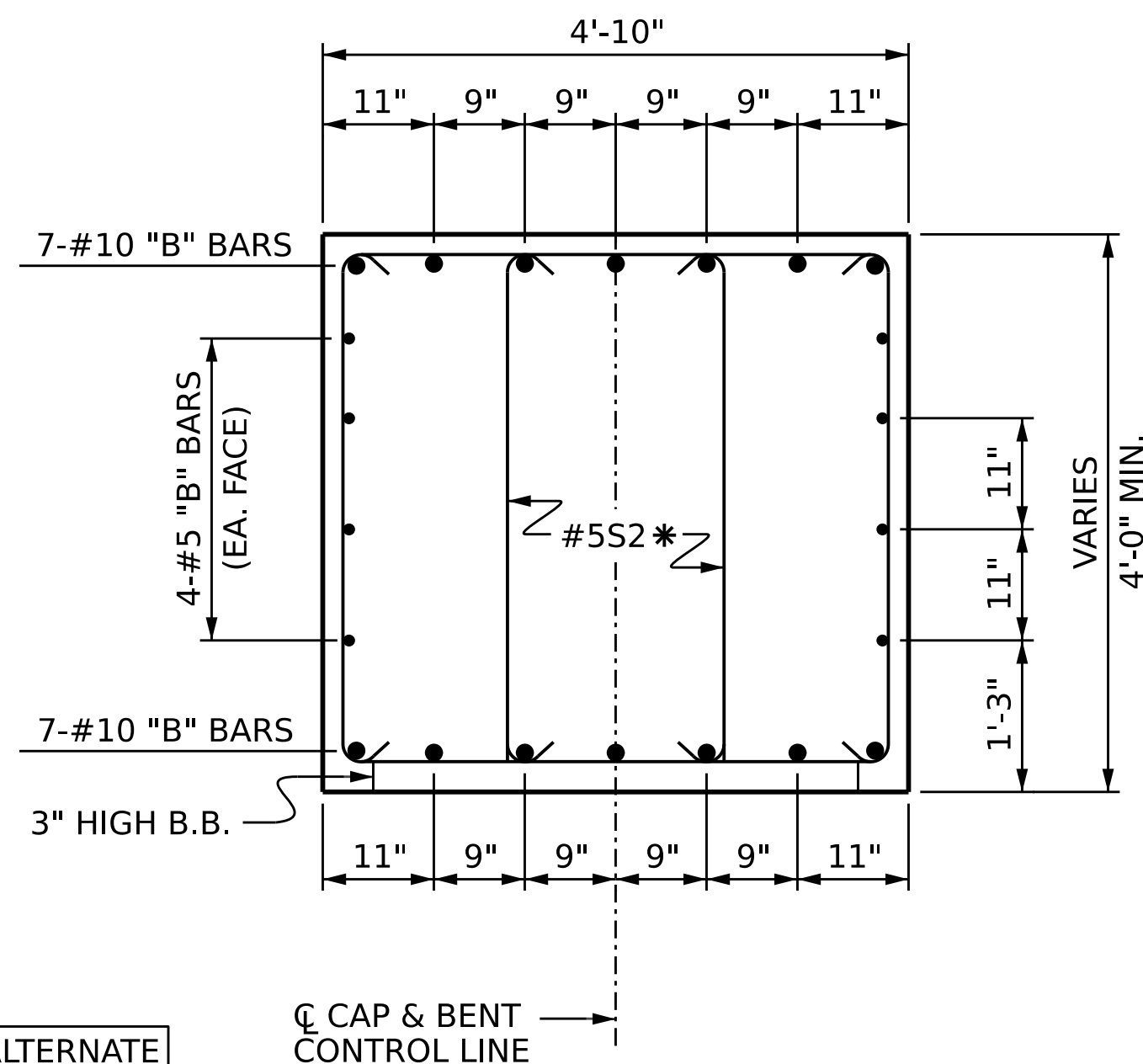
SECTION B-B
