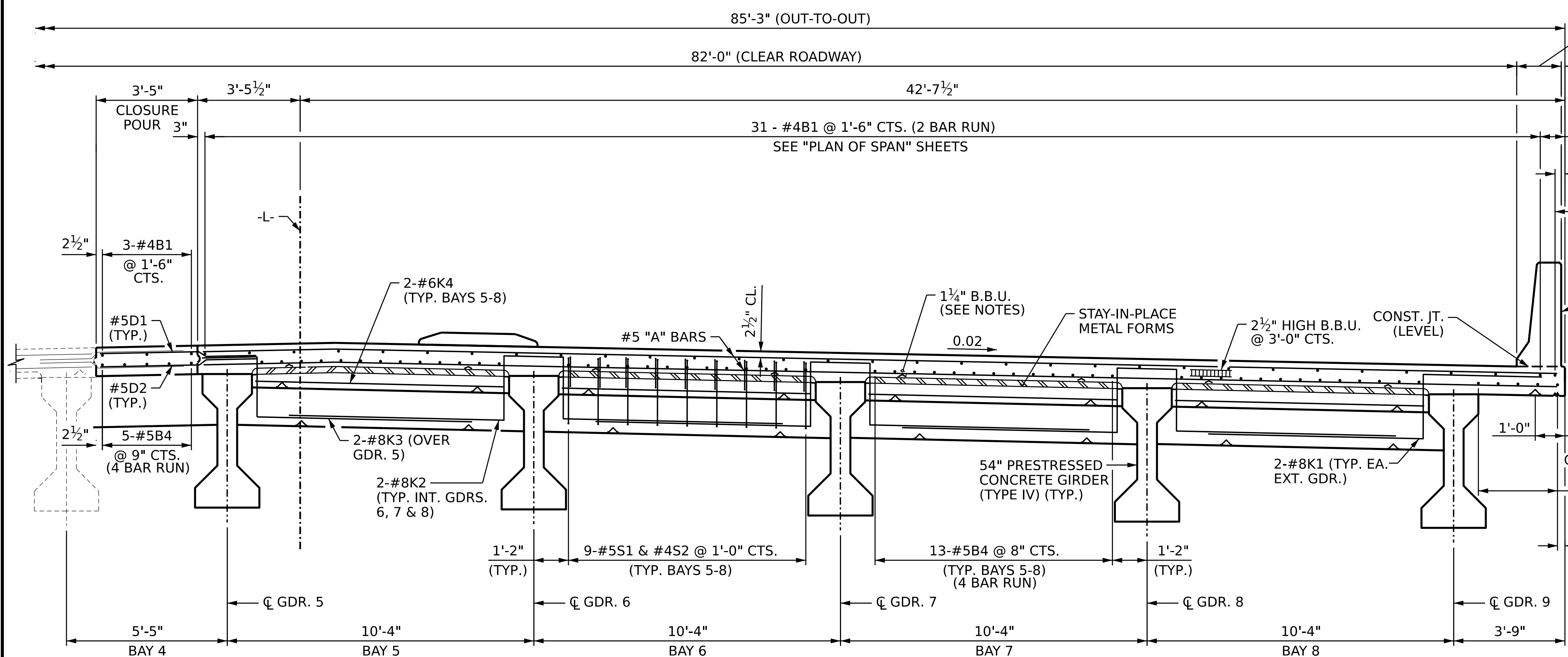
TYPICAL SECTION AT LINK SLAB
