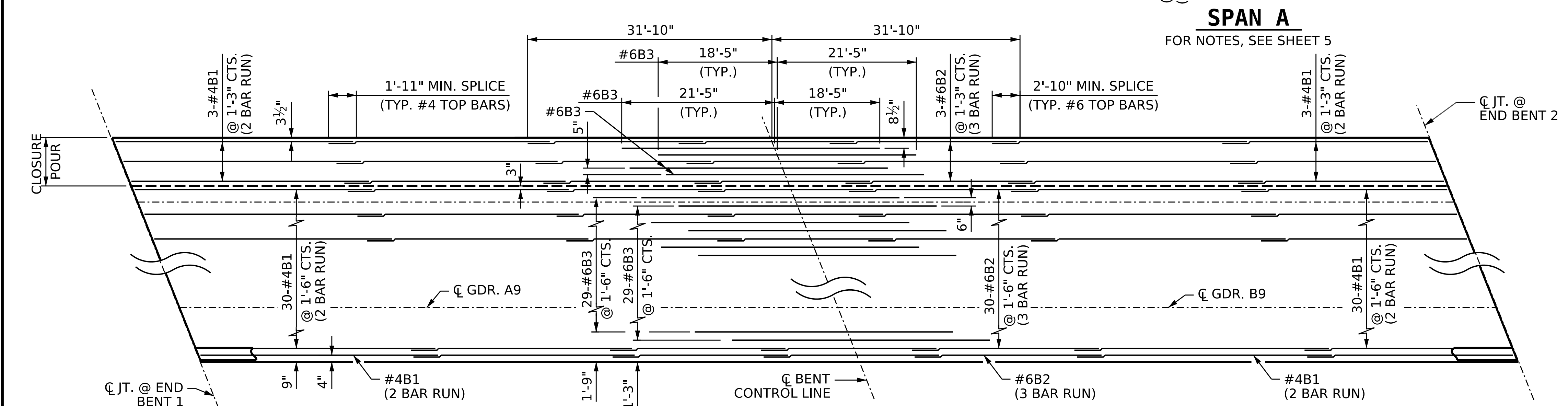
TOP REINFORCING STEEL LAYOUT SHOWING "B" BARS IN TOP OF SLAB (NOT DRAWN TO SCALE)
