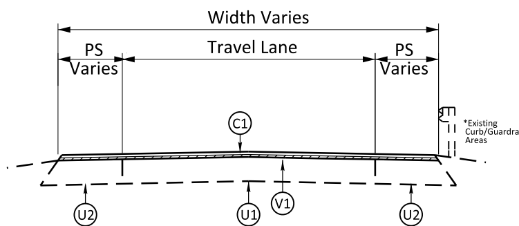
TYPICAL SECTION NO. 10 MAP 10
