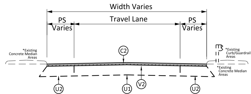
TYPICAL SECTION NO. 15 MAP 24
