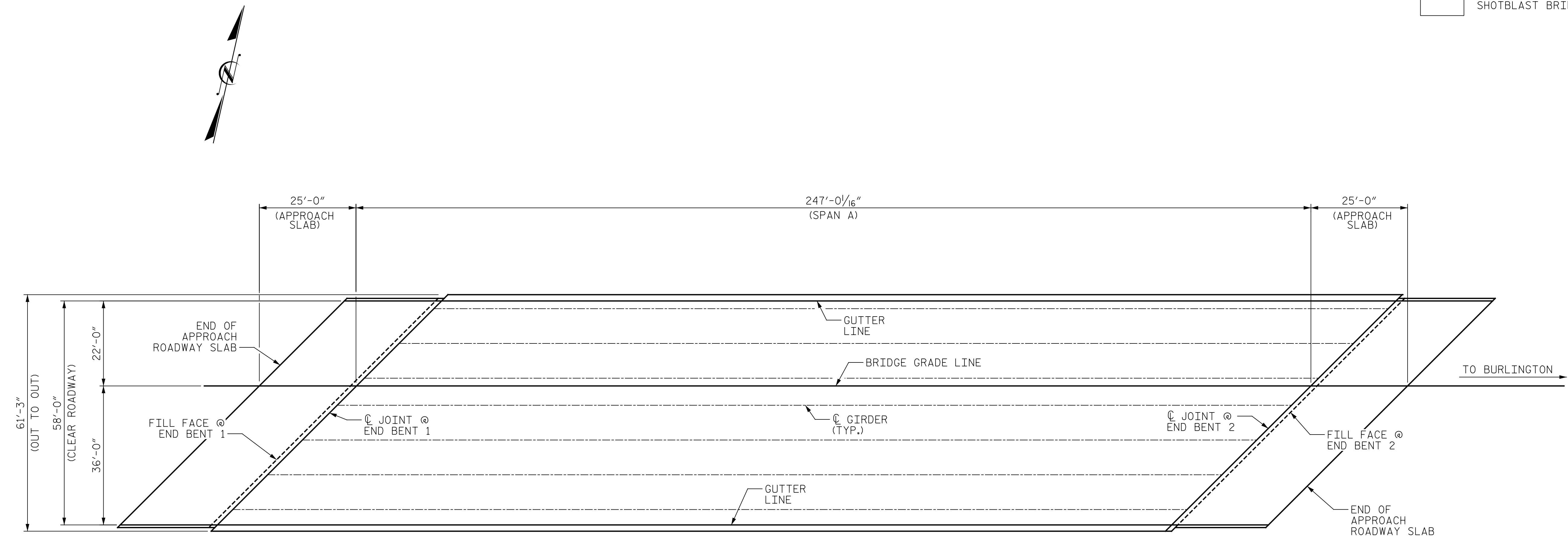
APPROACH SLAB @ END BENT 1 SPAN A APPROACH SLAB @ END BENT 2 PLAN
