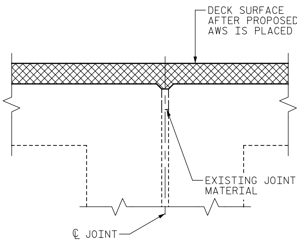
EXISTING JOINT AFTER AWS PLACEMENT
