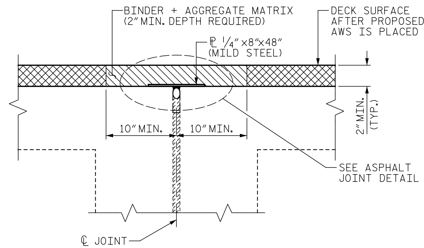
PROPOSED JOINT
