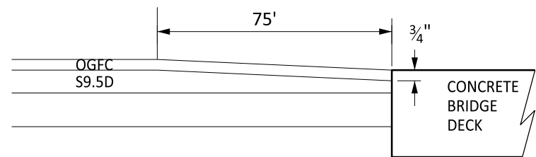
INCIDENTAL MILLING PAVEMENT DETAIL AT CONCRETE BRIDGES
