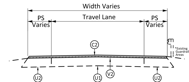
TYPICAL SECTION NO. 8 MAP 4, 6A, 7, 8, 17
