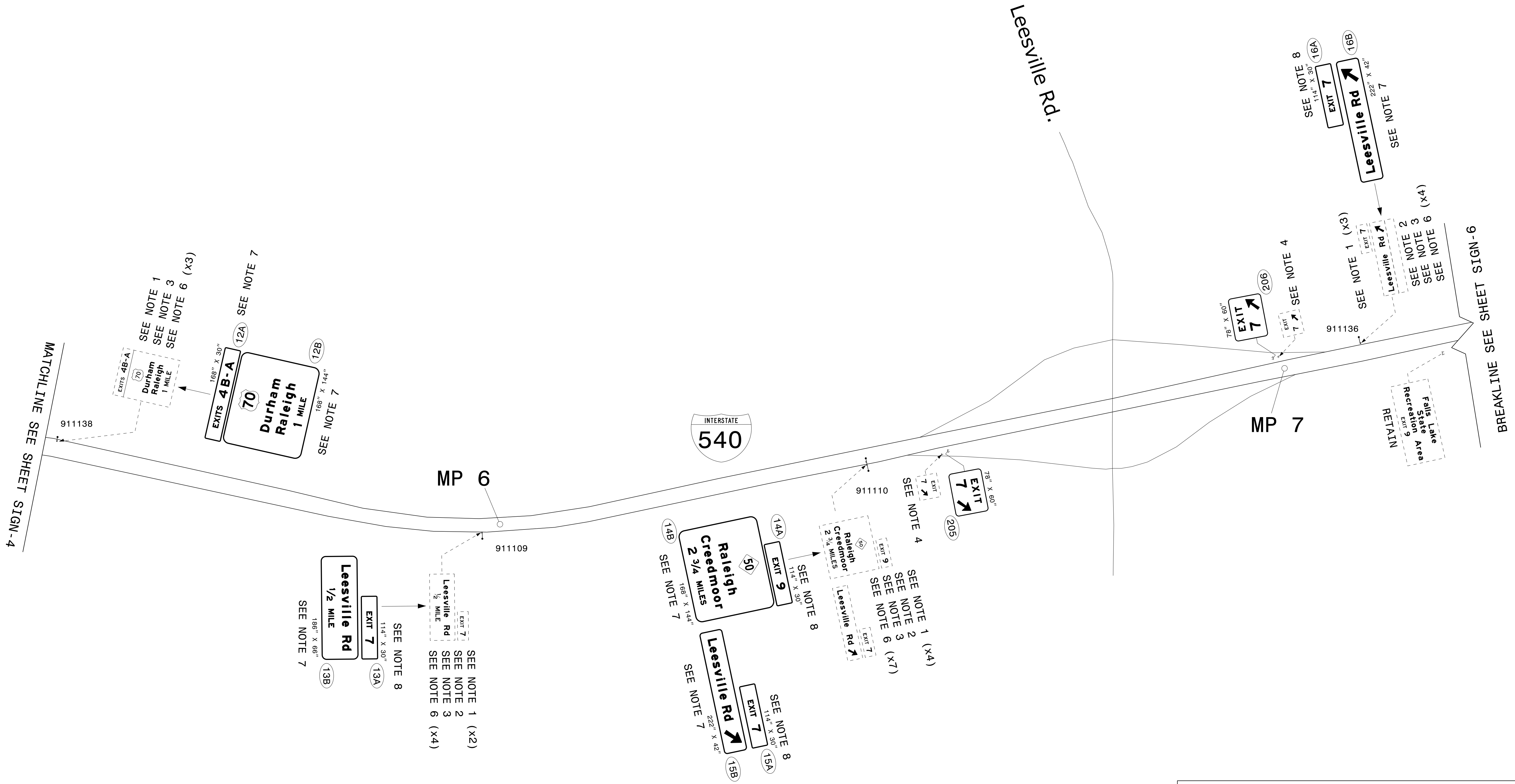
EXISTING AND PROPOSED SIGNS I-540
