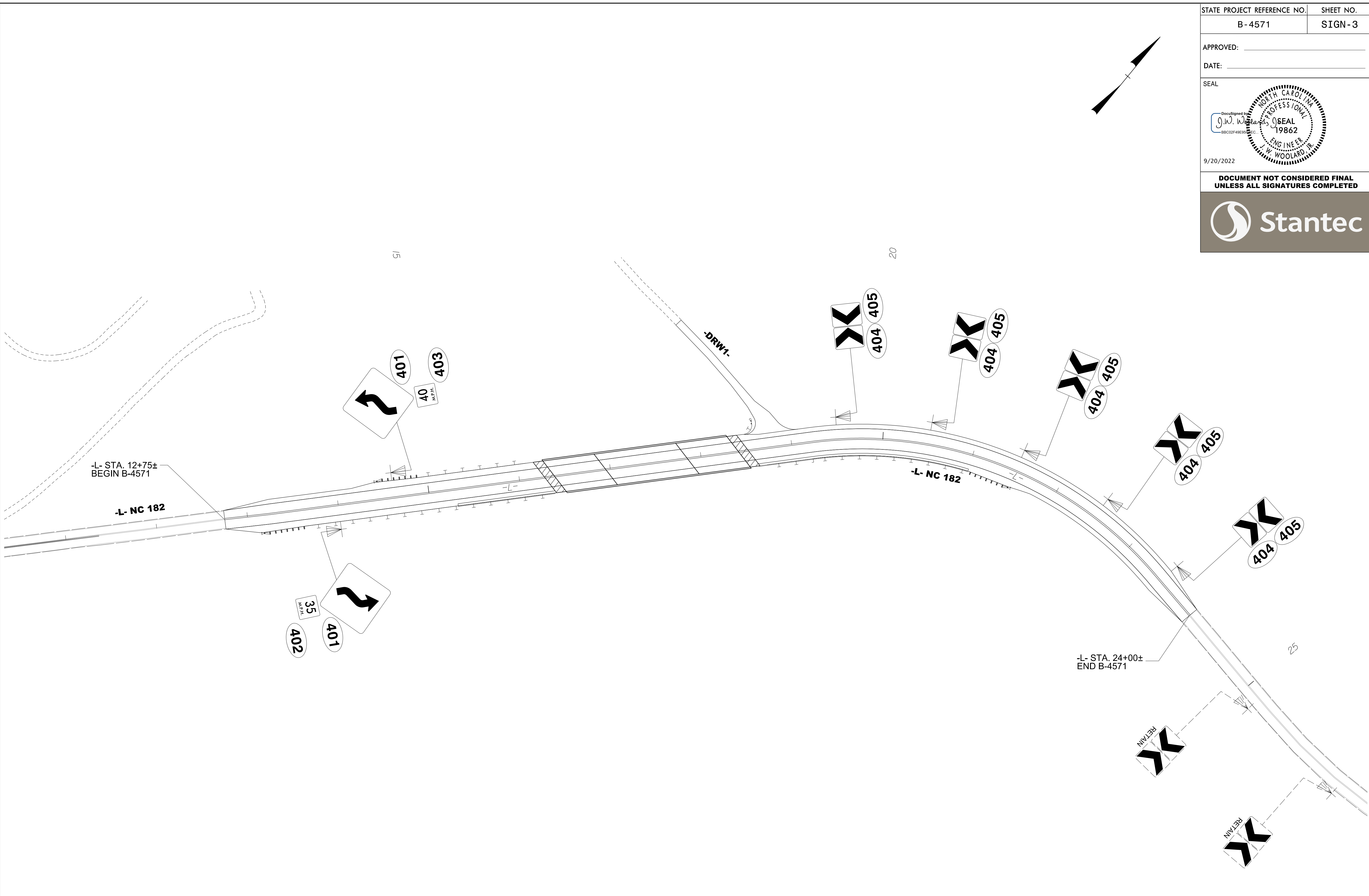
PROPOSED SIGNING DETAIL
