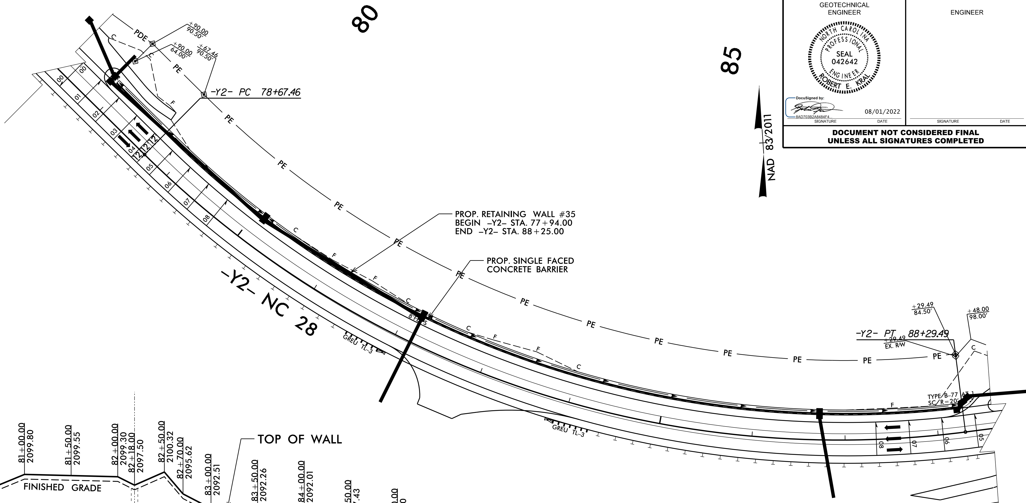
RETAINING WALL #35 - PLAN
