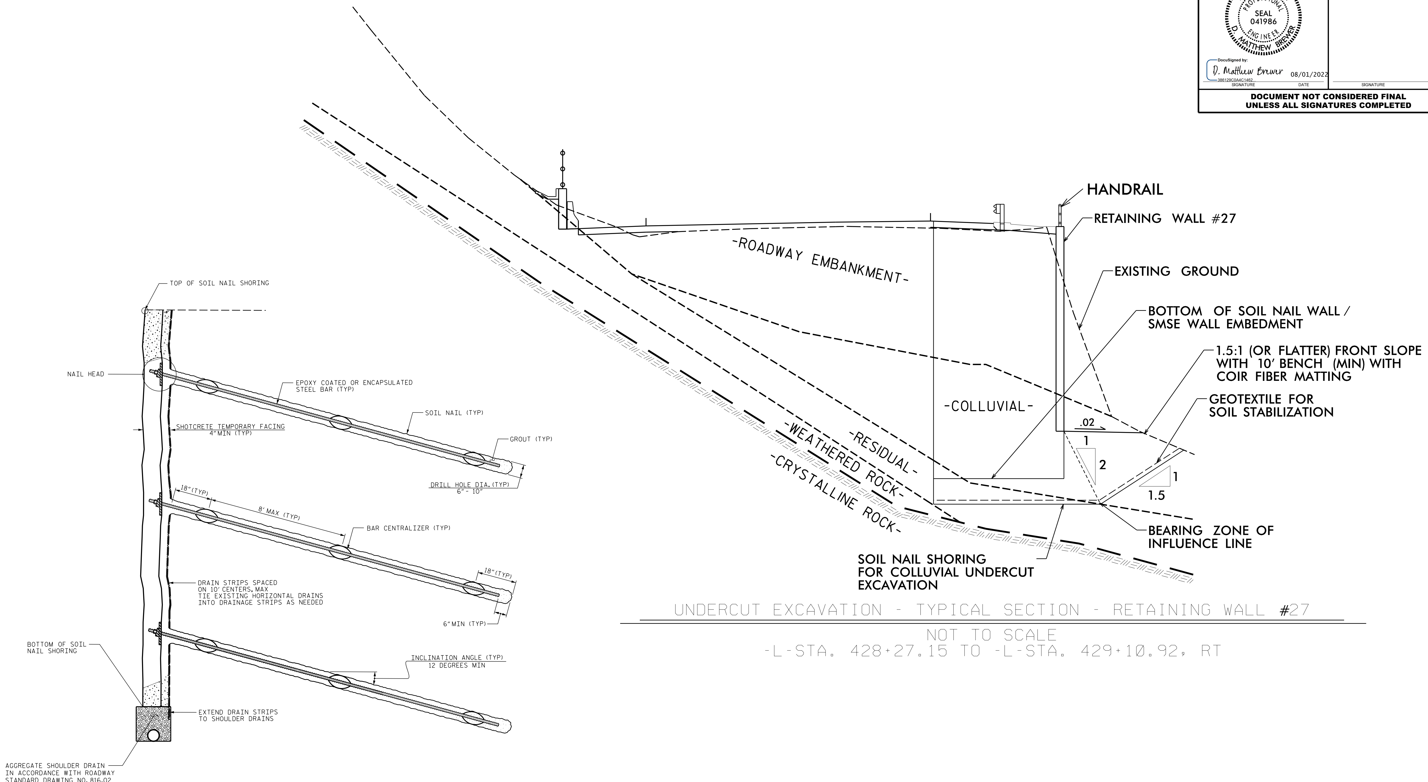
SOIL NAIL SHORING - TYPICAL SECTION NOT TO SCALE
