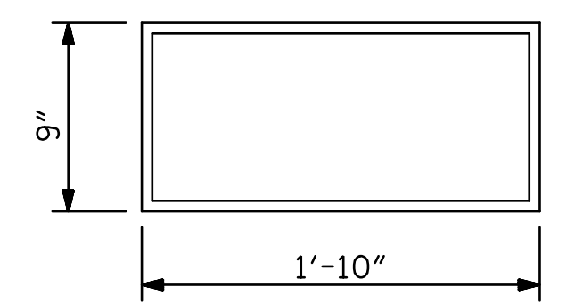
E3 (12 REQ'D) PLAN VIEW OF ELASTOMERIC BEARING TYPE IV
