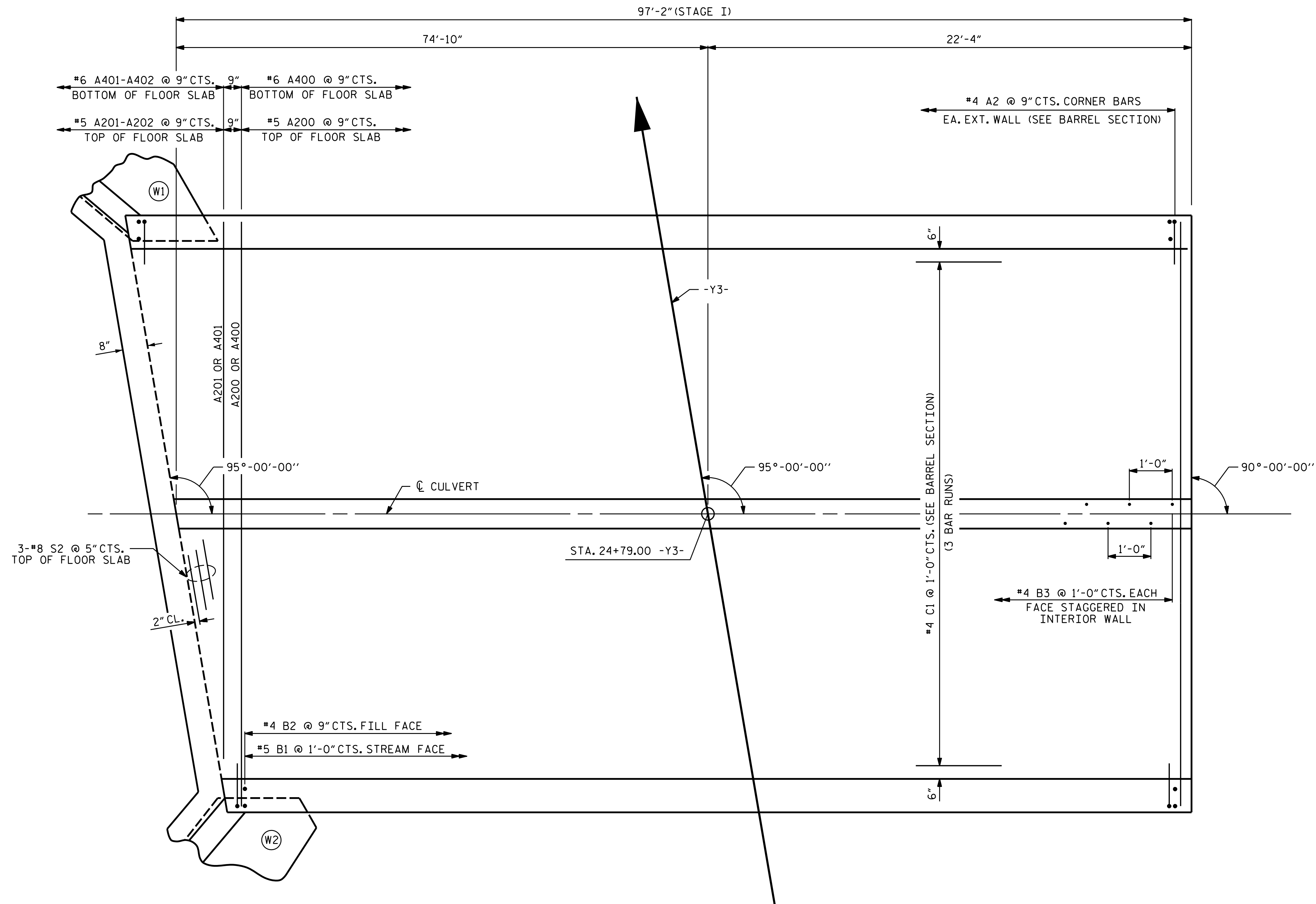
PLAN - FLOOR SLAB STAGE I FOR S1 BARS IN FLOOR SLAB & FOOTING, SEE WING SHEET.
