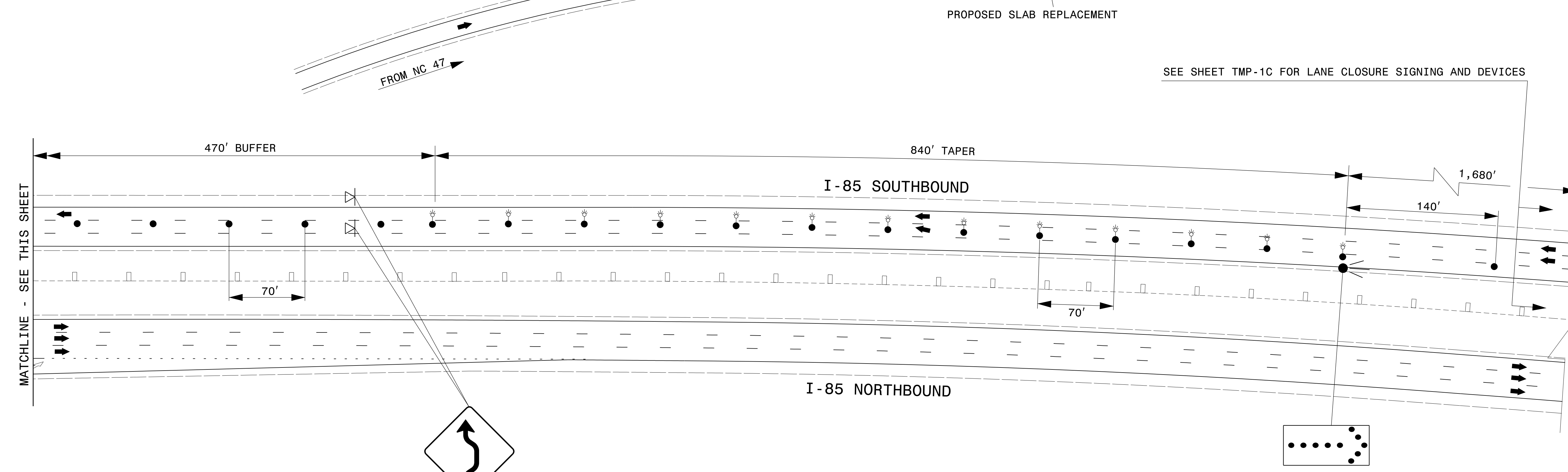
W24-1R 48" X 48" PLACE JUST INSIDE OF SINGLE-LANE BUFFER ZONE
