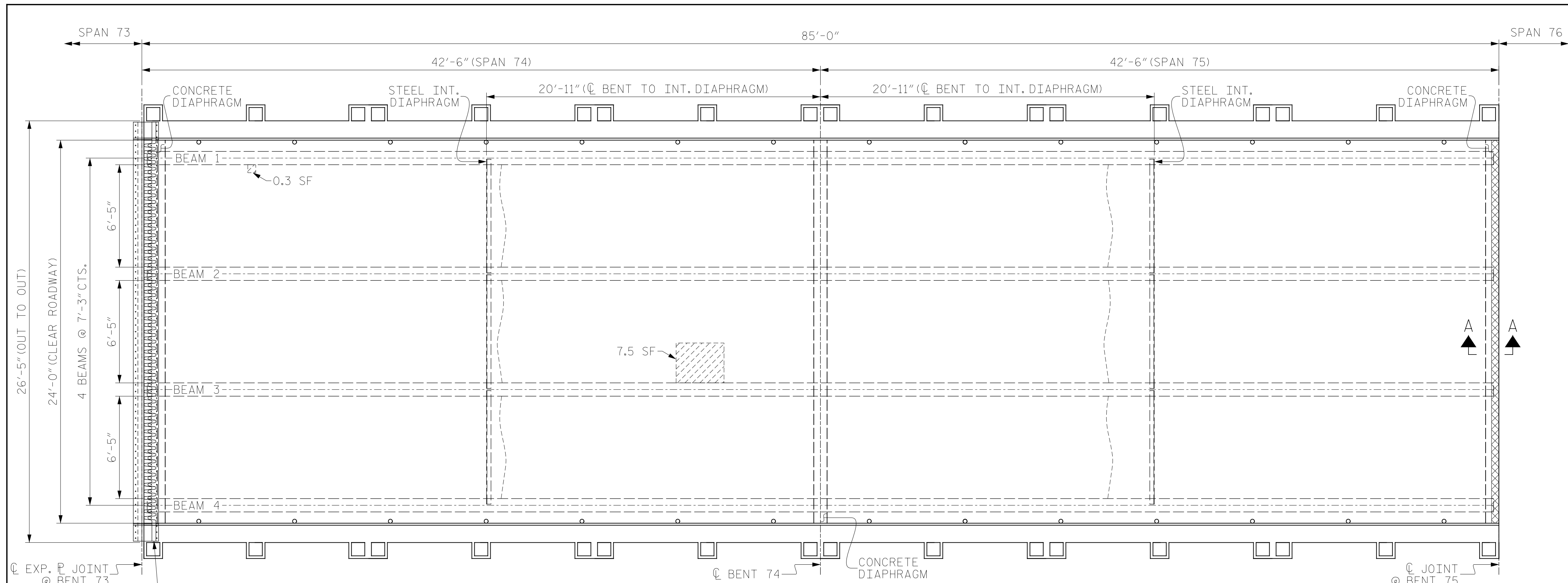
PLAN OF SPAN 74
