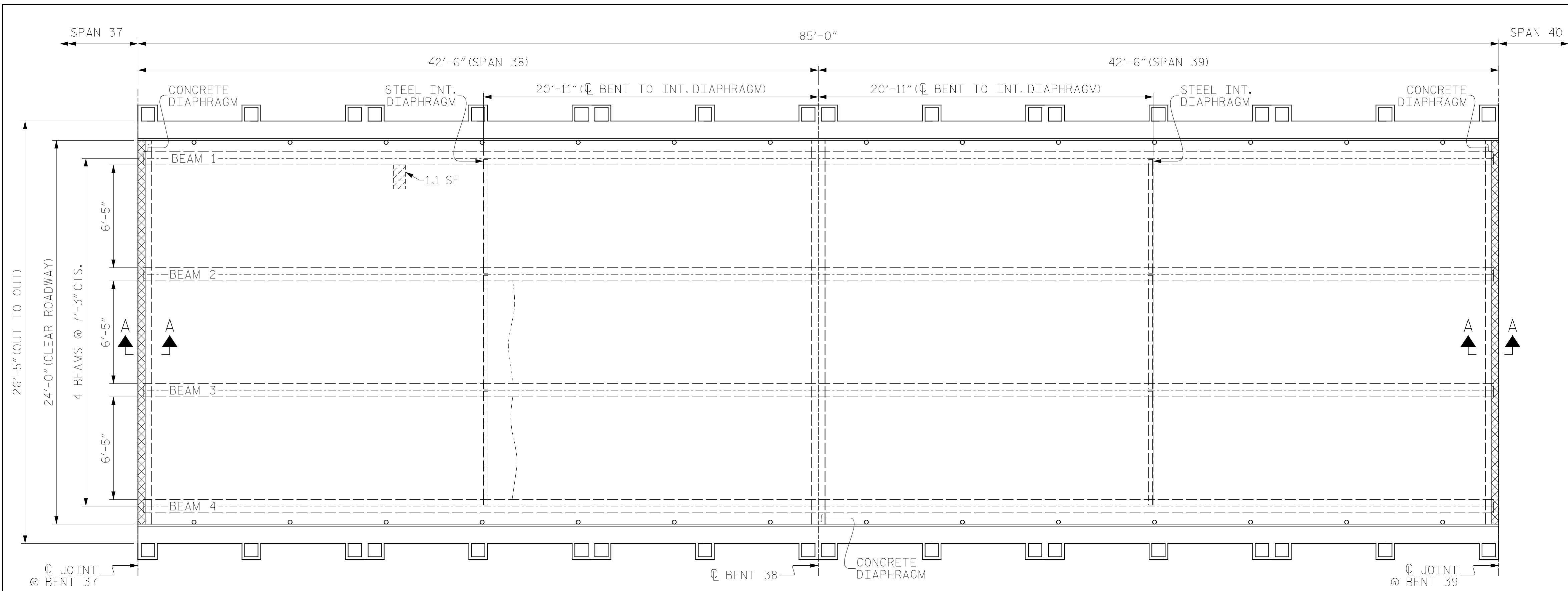
PLAN OF SPAN 38
