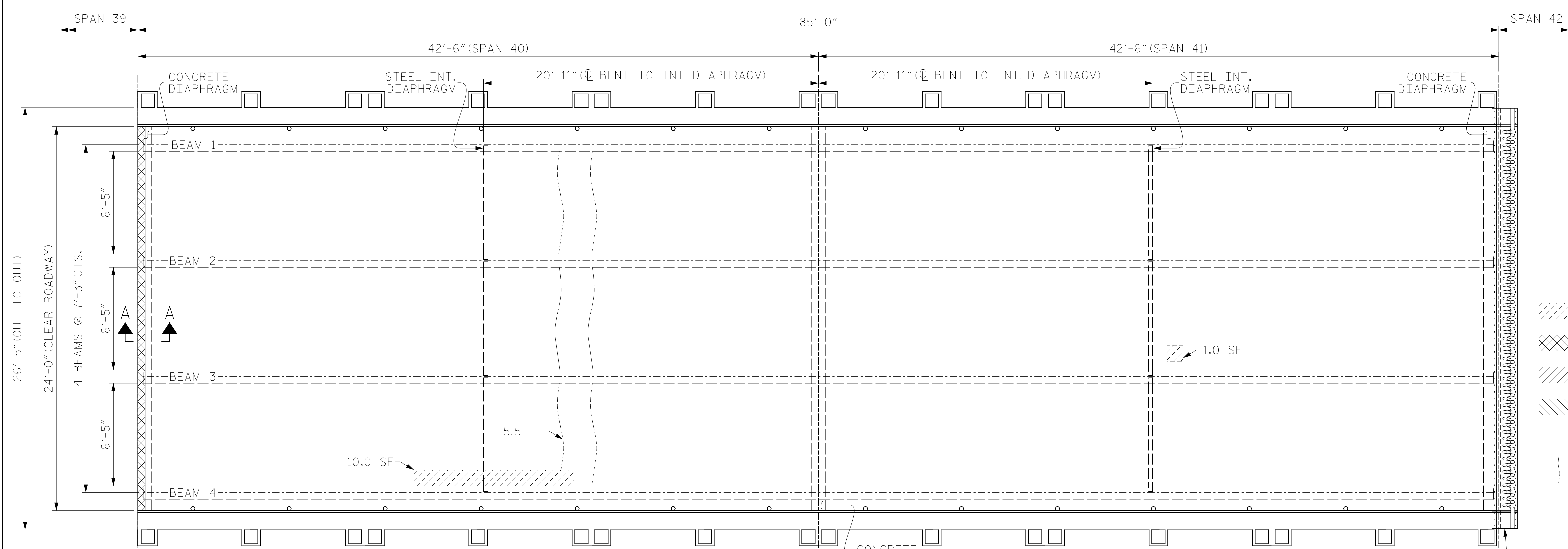
PLAN OF SPAN 40
