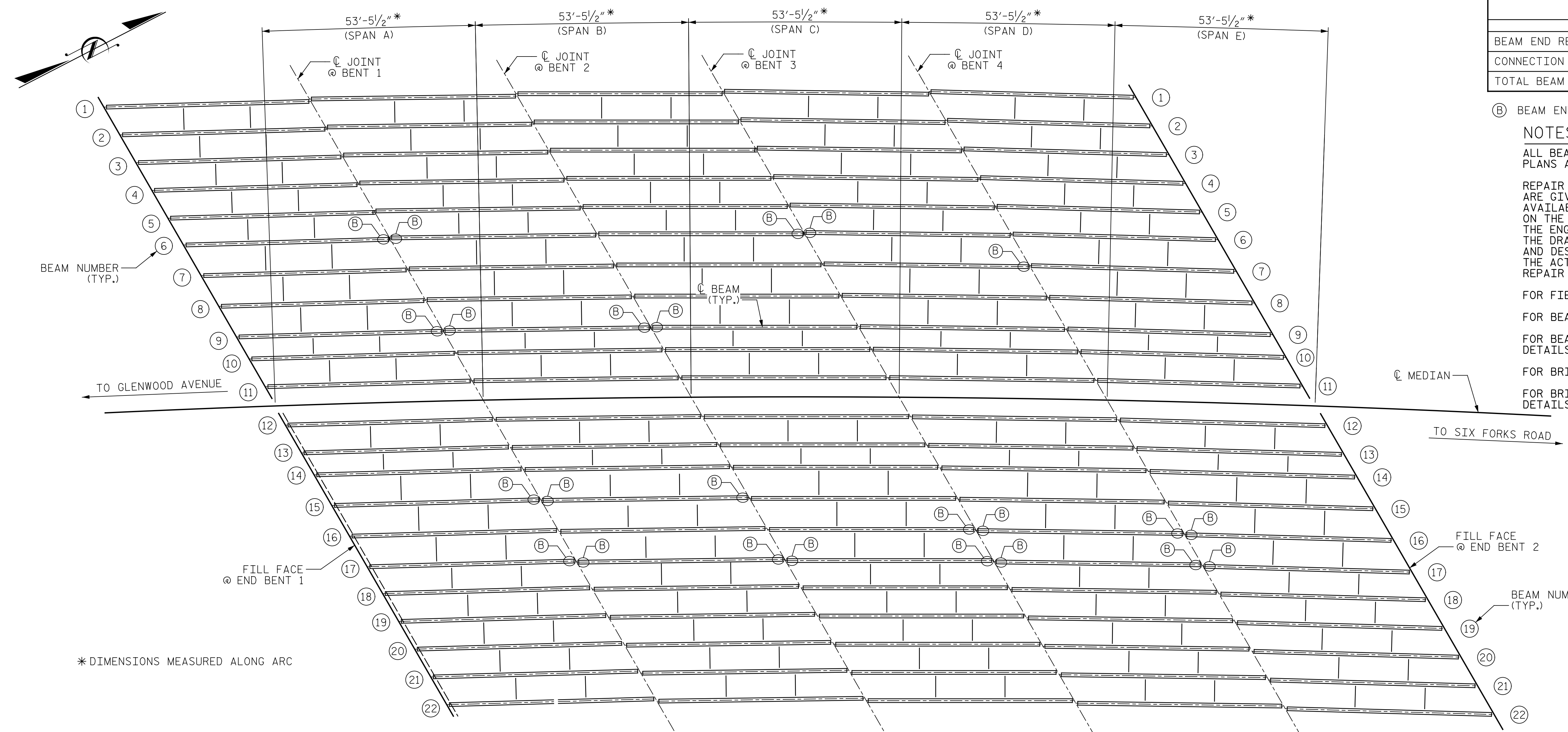
BEAM REPAIR LOCATIONS (OTHER LOCATIONS MAY EXIST, SEE NOTES)
