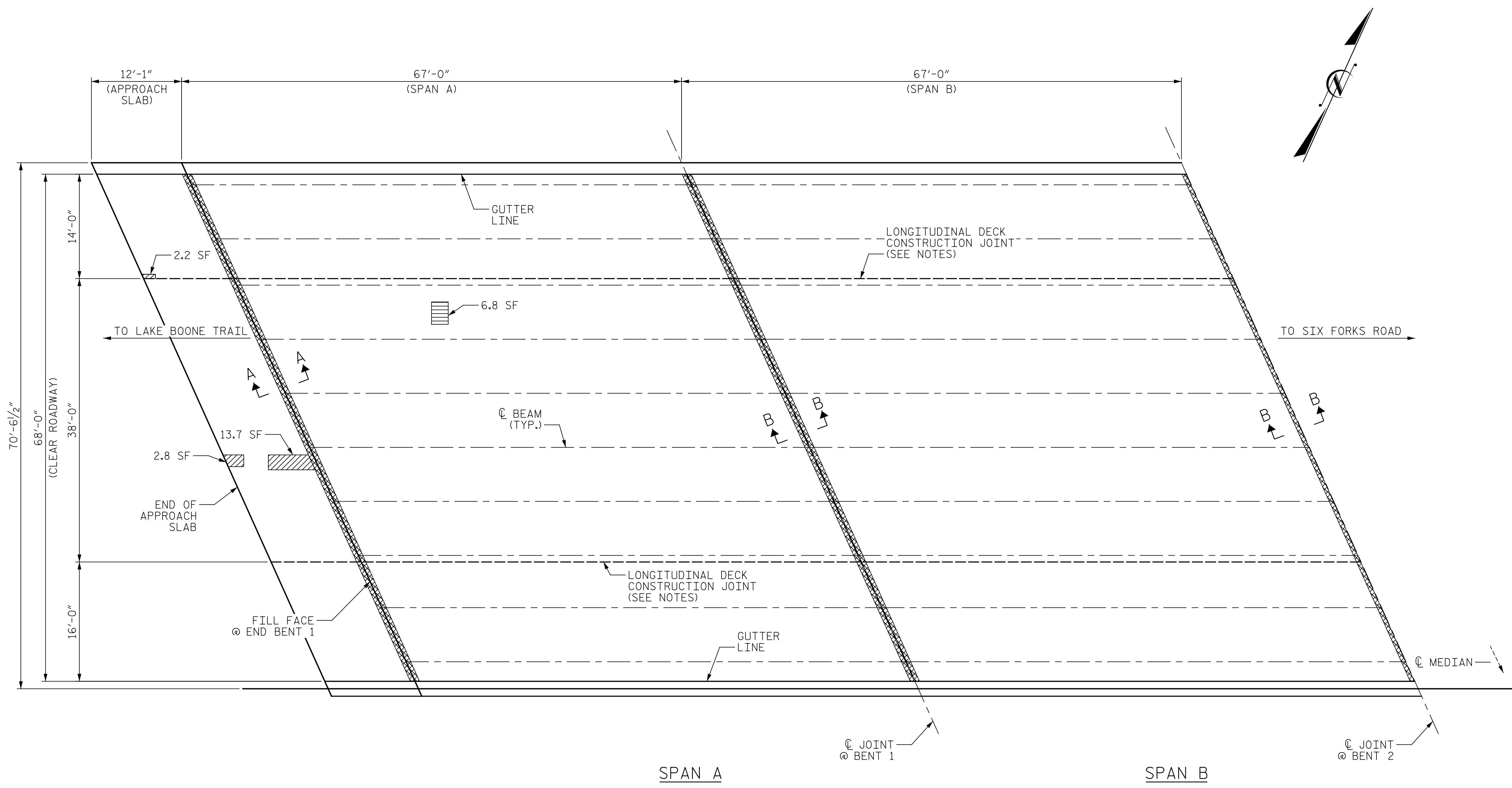
PLAN
