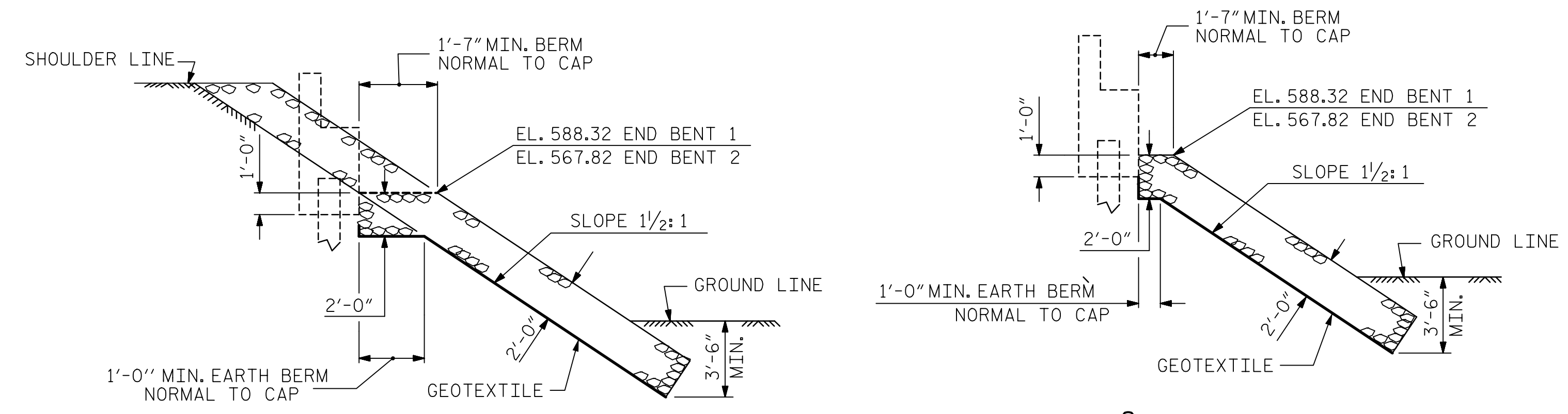
SECTION H-H
