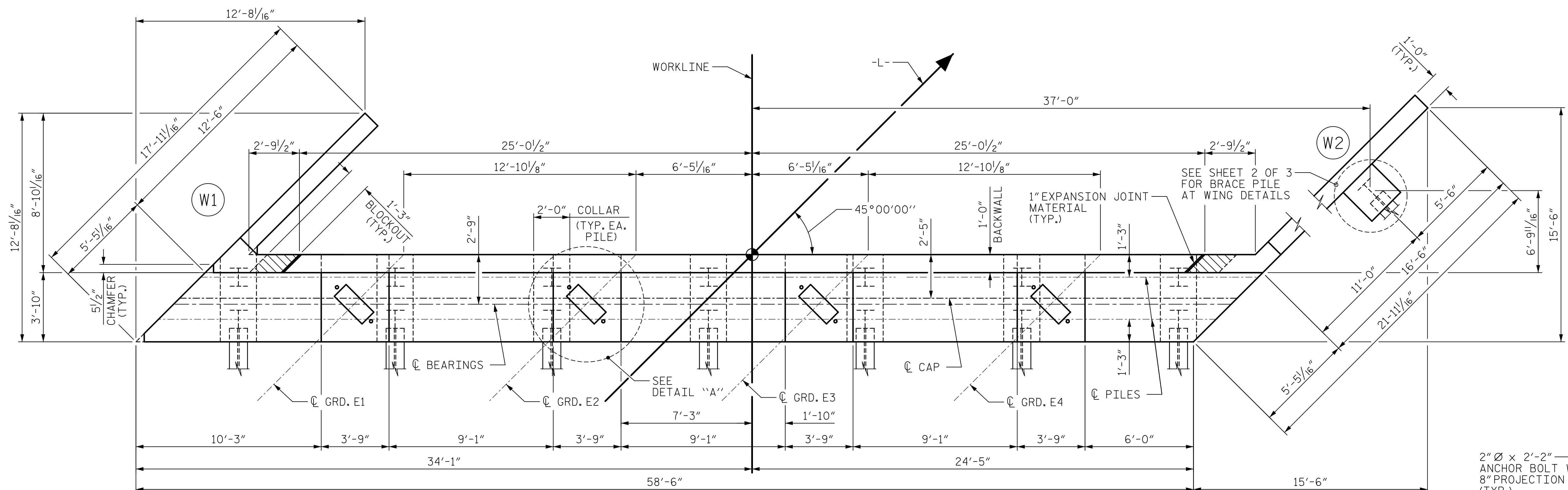
PLAN
