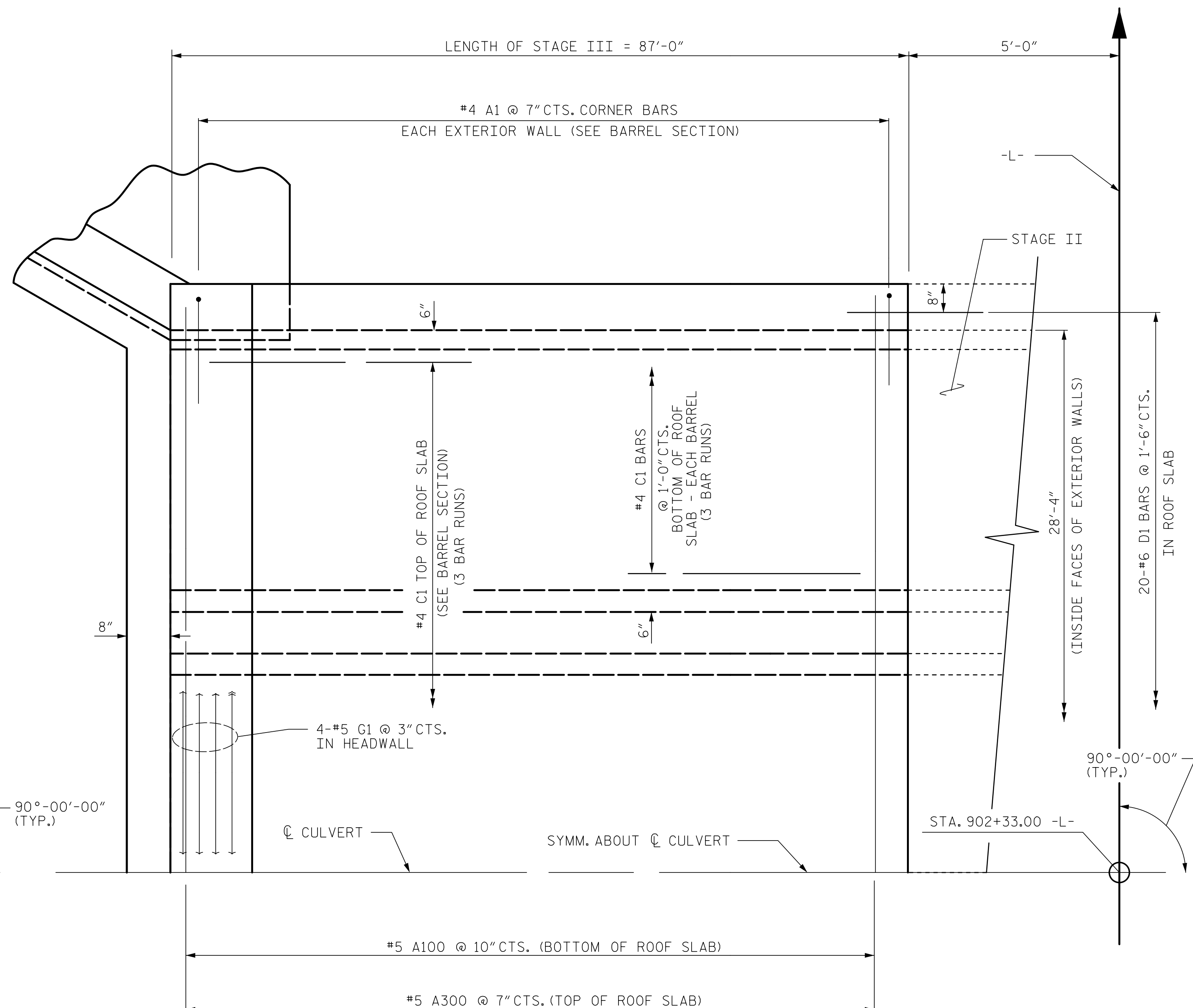
PART PLAN - ROOF SLAB
