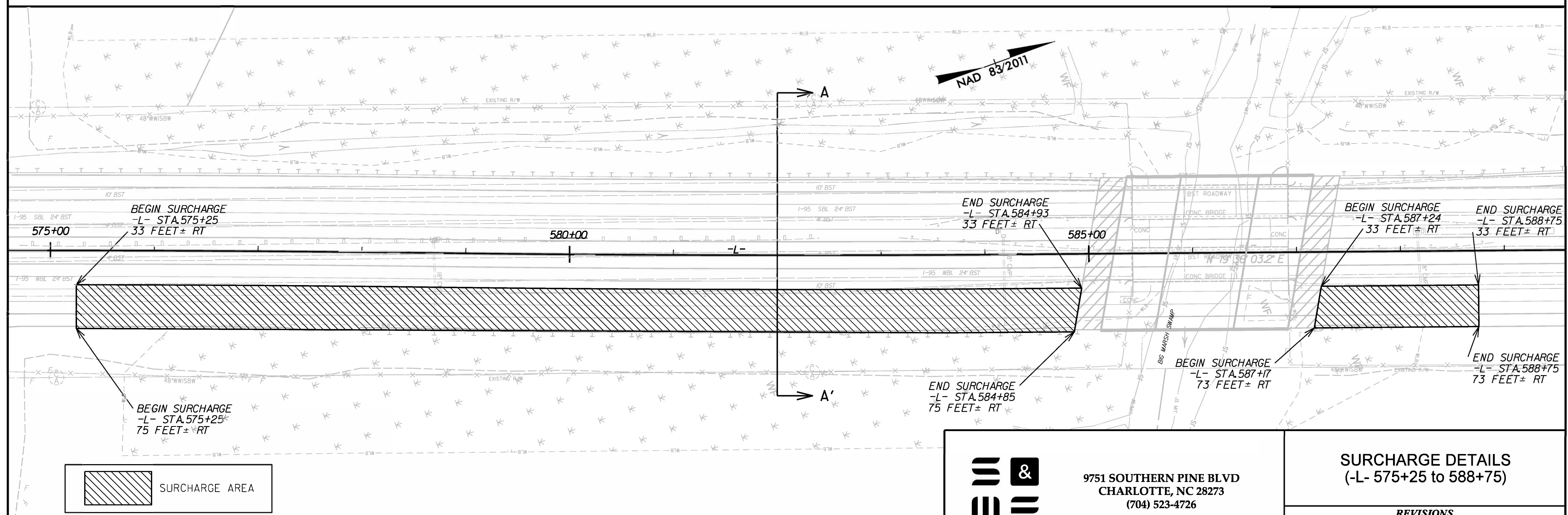
PLAN VIEW FOR SURCHARGE
