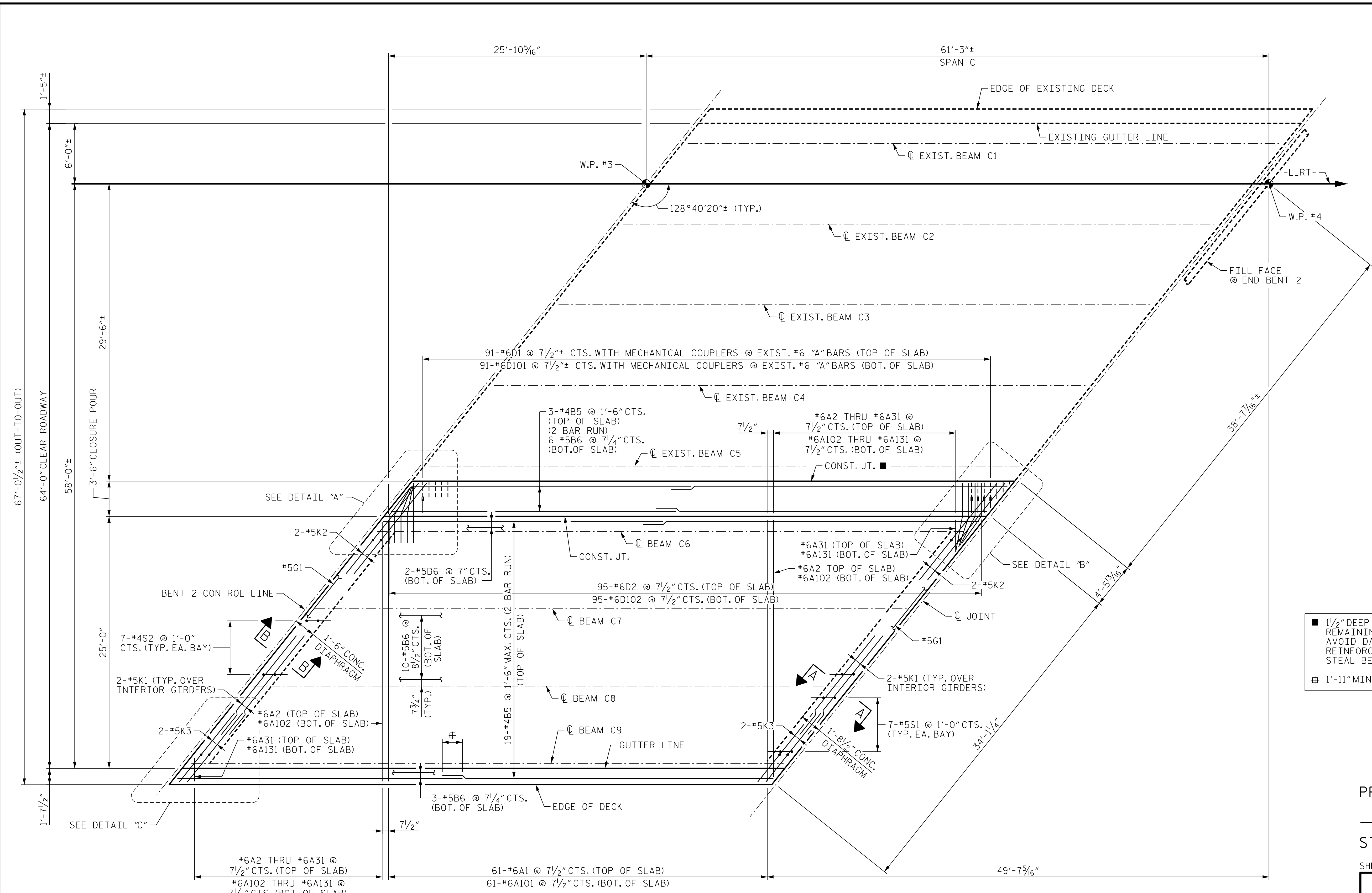
PLAN OF SPAN C
