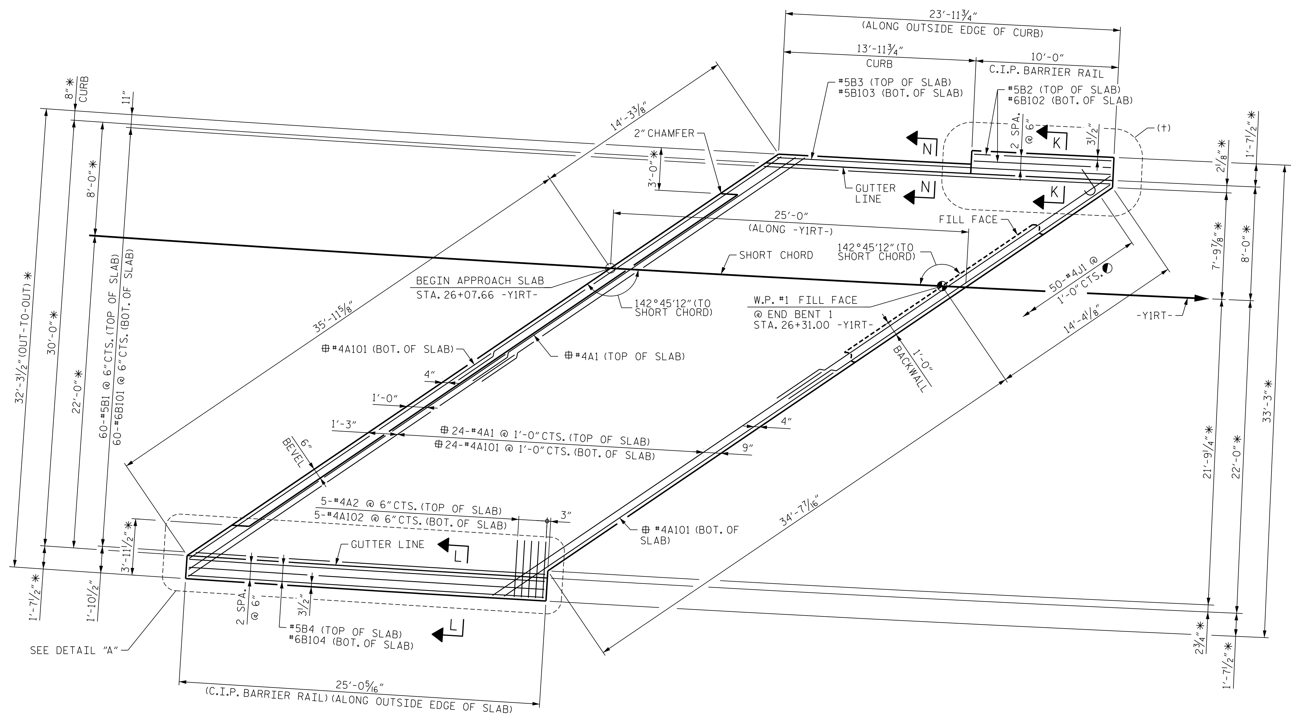
PLAN OF APPROACH SLAB AT END BENT 1
