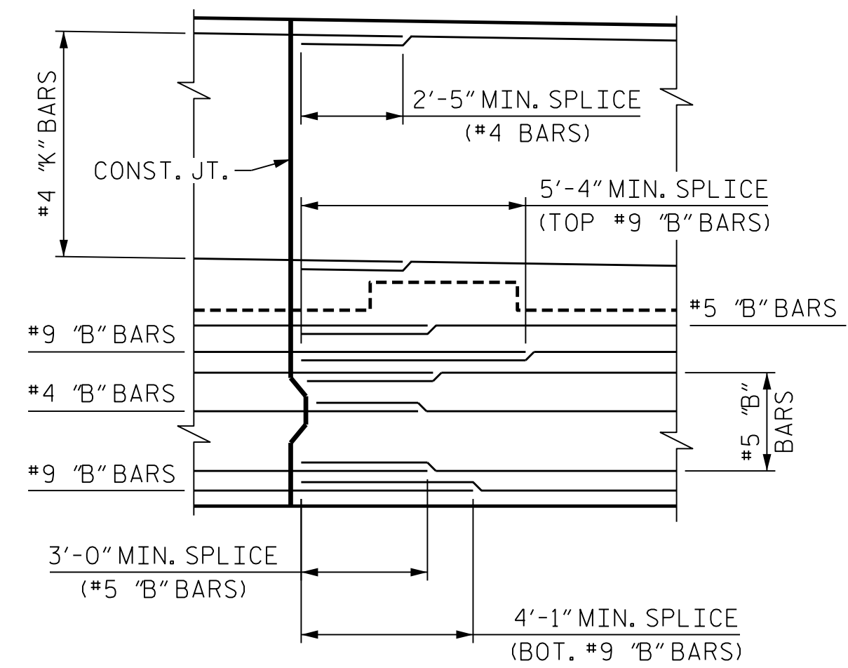
SPLICE DETAIL
