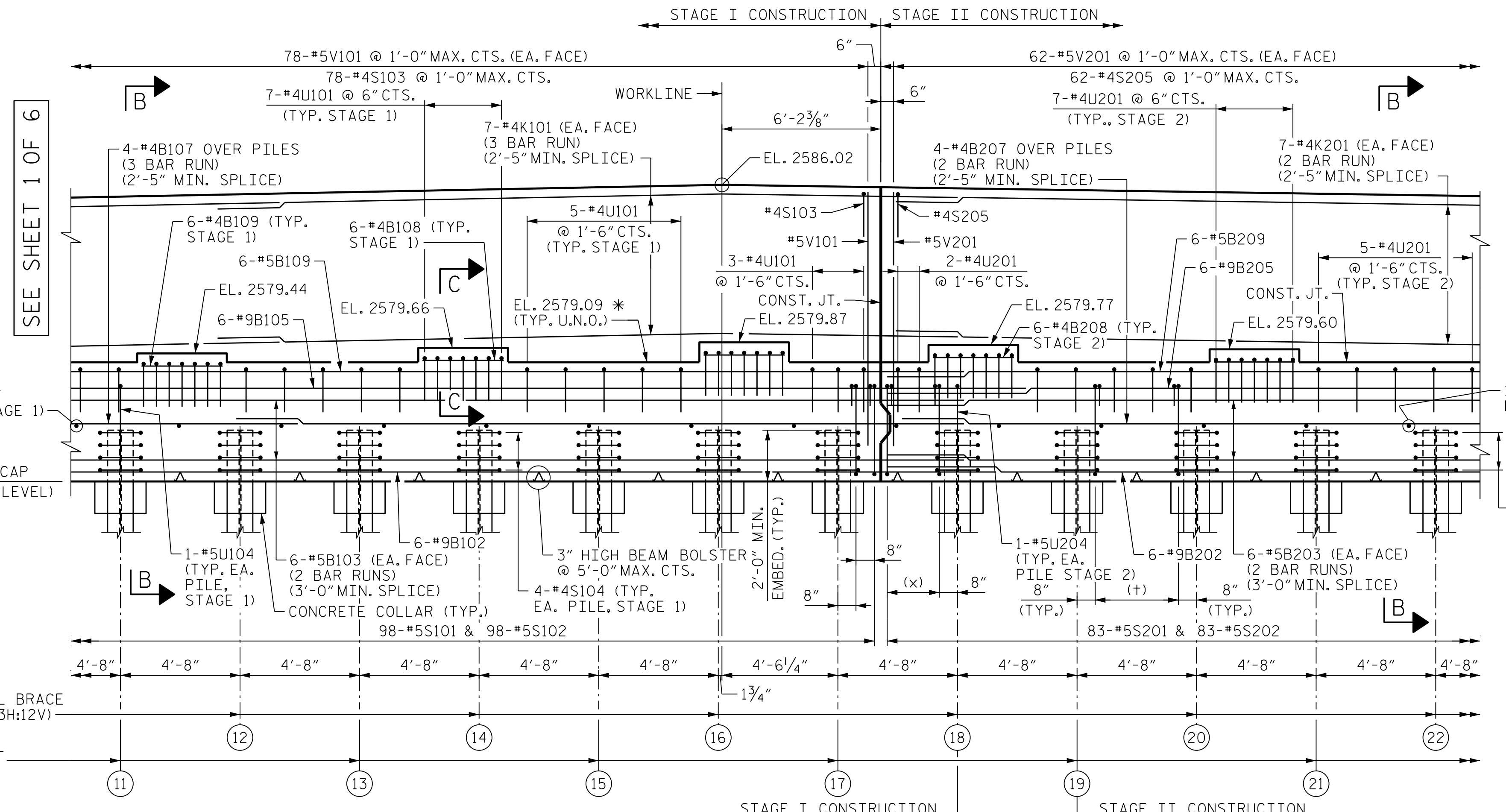
PARTIAL ELEVATION
