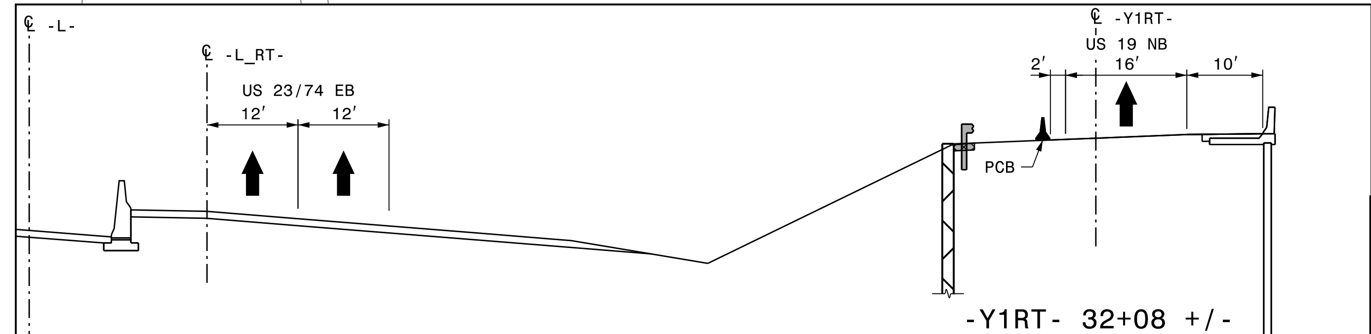
SECTION F-F -L- 54+50
