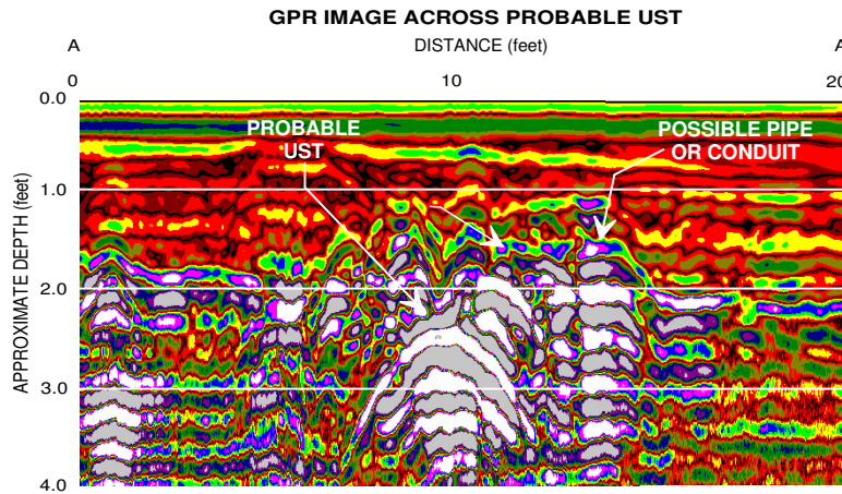
GPR scanning across the EM61 differential anomaly centered near UTM coordinates 986027.5-E 12920801.5-N yielded high amplitude, hyperbolic reflections in the GPR image shown above. The GPR anomaly is probably in response to a metallic UST buried approximately 2.2 feet below present grade. The purple line labeled AA' in the photograph shown below represents the approximate location of the GPR image.
