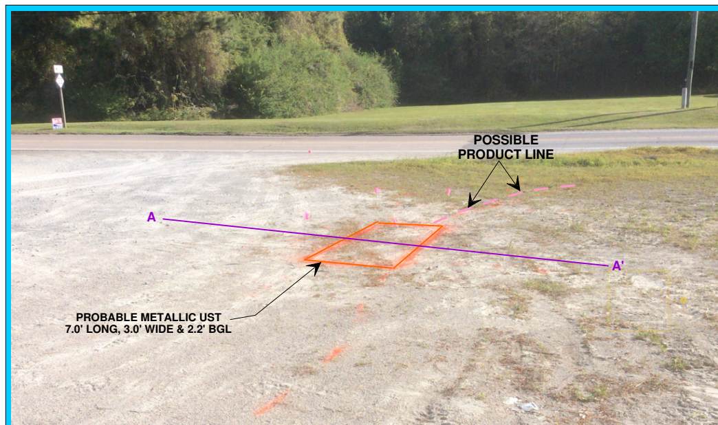
The orange rectangle in the photograph represents the approximate foot print of a probable UST that was detected by the geophysical investigation. Based on the GPR data, the UST is approximately 7.0 feet long, 3.0 feet wide and buried 2.2 feet below present grade. The solid purple line labeled AA' in the photograph represents the approximate location of GPR image AA' shown above. The dashed pink line represents the approximate location of a possible product line that runs from the UST in a northerly direction. The photograph is viewed in a northerly direction.
