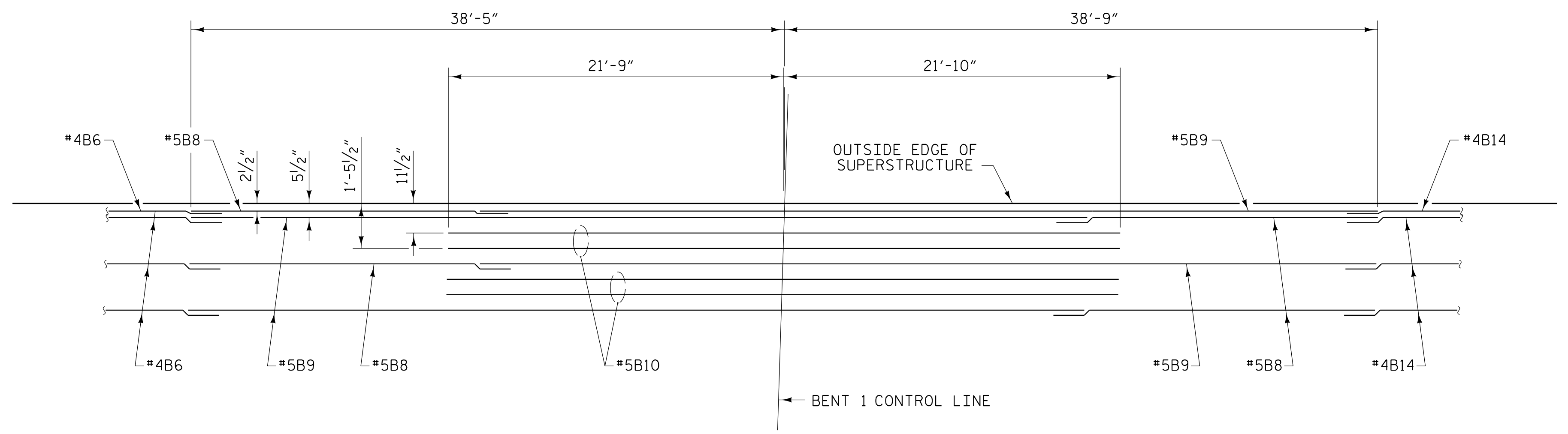
TOP OF DECK "B" BAR PLACEMENT AT BENT 1
