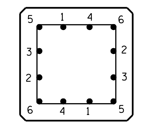
TYPICAL PATTERN FOR BURNING STRANDS
