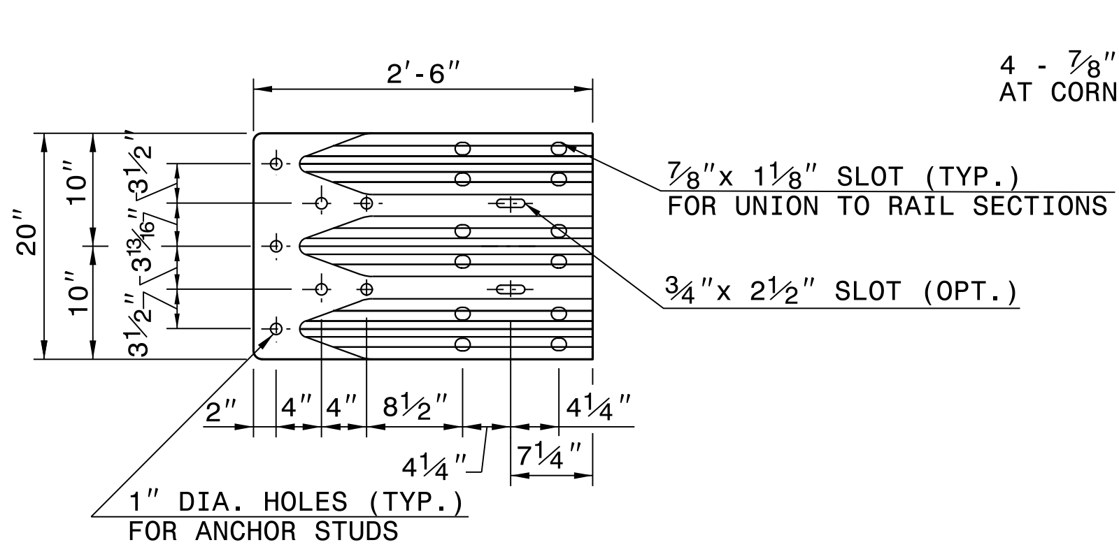
END SHOE
