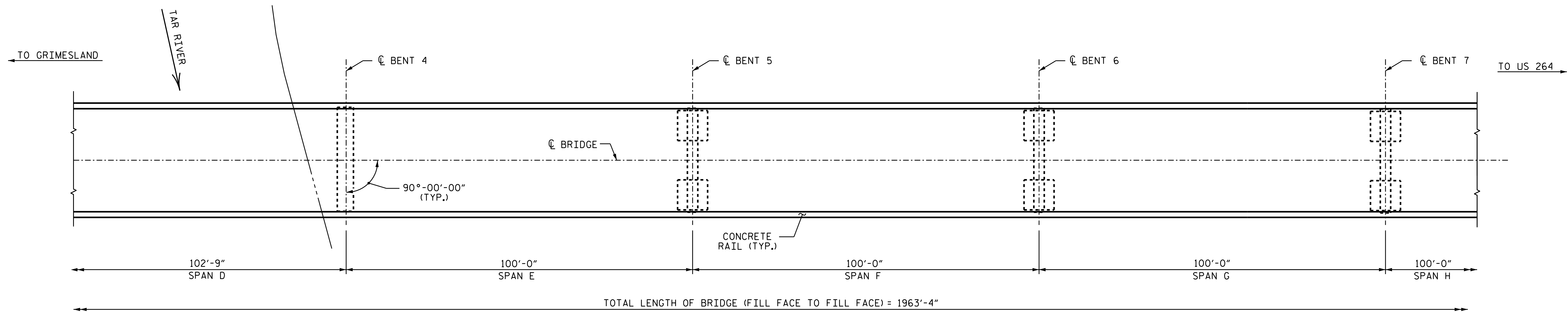
PLAN (PILES, COLUMNS, AND DRILLED PIERS NOT SHOWN FOR CLARITY)
