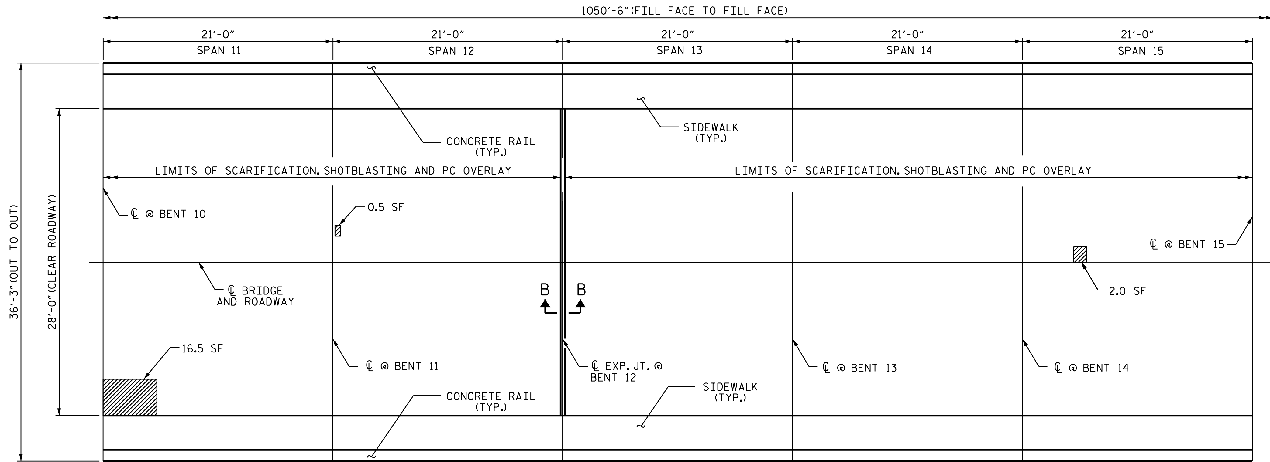
PLAN (SPANS 11 THRU 15)
