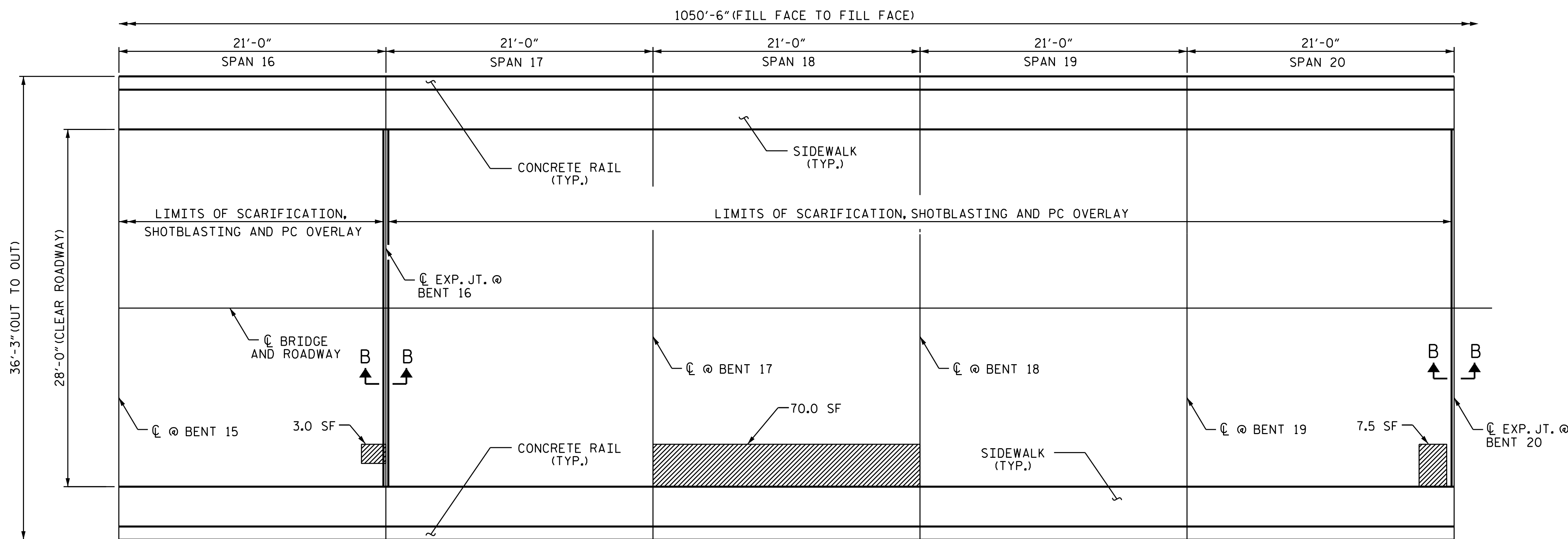
PLAN (SPANS 16 THRU 20)
