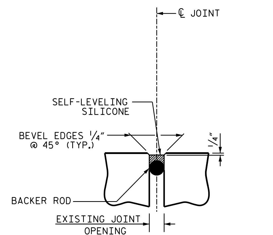
PROPOSED JOINT SEAL DETAIL
