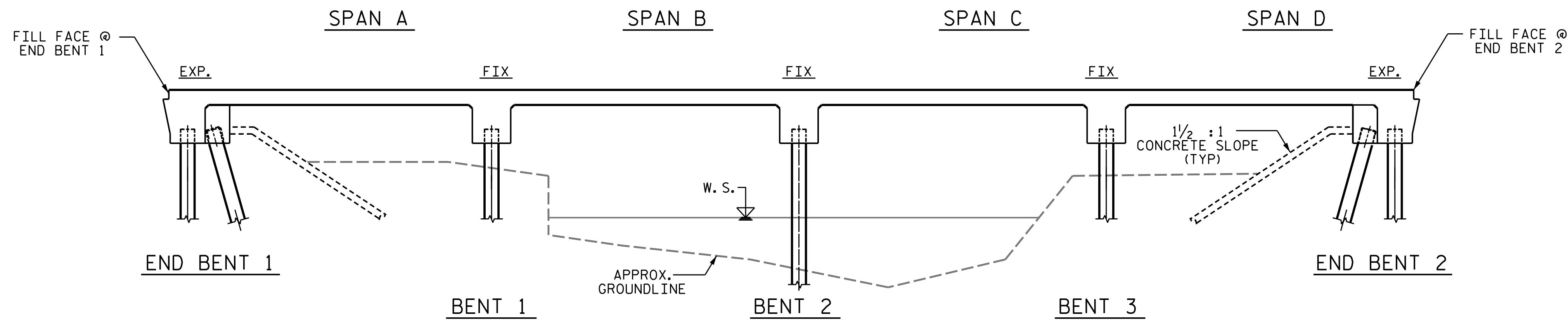
ELEVATION (SECTION ALONG \bar{C} ROADWAY)
