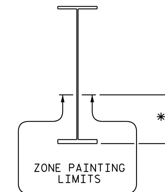
DETAIL B (ADDITIONAL BEAM AREA)
